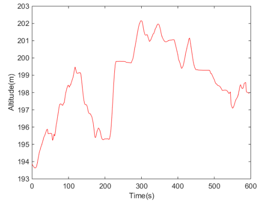
Figure 19. Scenario 7 true vertical trajectory
