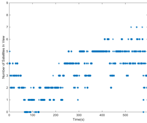
Figure 36. Scenario 7 number of SVs viewable vs time.
