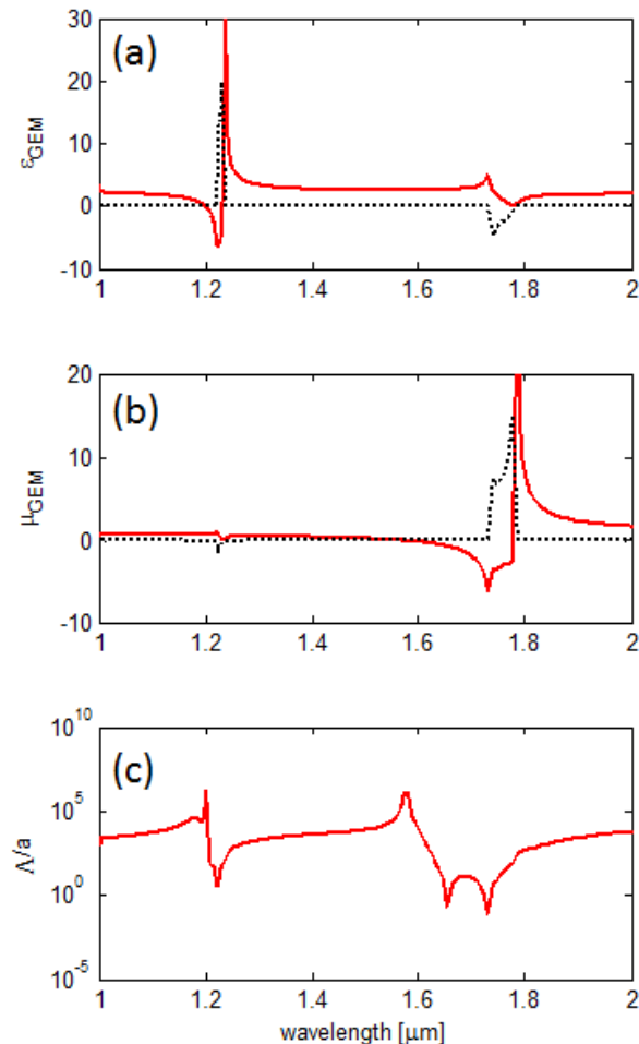
Figure 6. Effective \epsilon (a) and \mu (b) from GEM model for spheres of radius 0.12 \mu\text{m} , with \epsilon_2=50 in vacuum ( \epsilon_1=1 ) with a loading density of 25%, and the mean-free path (normalized to a ) for 1% vacancy density (c).
