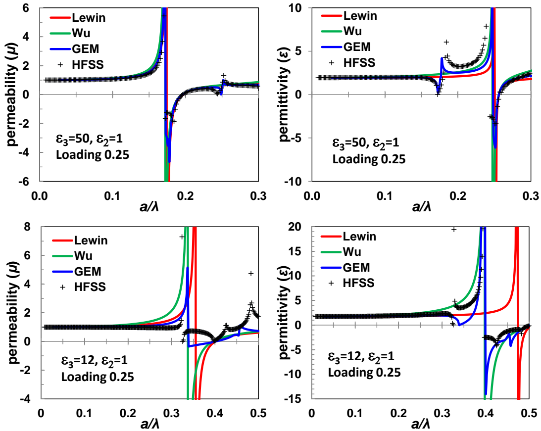
Figure 2. Comparison of calculated \text{Re}(\mu) and \text{Re}(\epsilon) versus a/\lambda for the GEM (blue), Wu (green), Lewin (red) models to HFSS (symbol) calculations. Top panel ( \epsilon_3=50 , \epsilon_2=1 ) and bottom panel ( \epsilon_3=12 , \epsilon_2=1 ).
