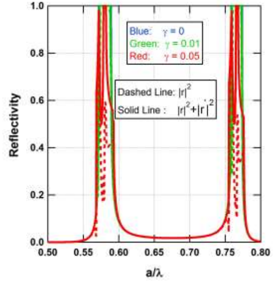
Figure 14. Reflectivity as a function of a/\lambda for a semi-infinite MM with different disorder strengths. Dashed and solid lines correspond to reflection along the same polarization direction as the incident light and the total reflection. Here, a is the lattice constant of an ordered simple cubic structure, \lambda is the wavelength, and \gamma is the disorder strength.
