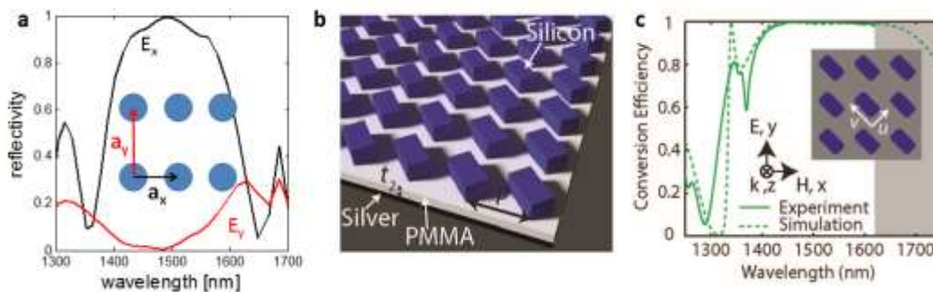
Figure 18. (a) Anisotropic unit cell and predicted spectral reflectivity for x -polarized (black) and y -polarized (red) light by a single layer of Si cylinders with radius of 0.2 \mu\text{m} , a_x=0.7 \mu\text{m} , and a_y=1.23 \mu\text{m} . Near 1.5 \mu\text{m} , light polarized along x is 100 % reflected and light polarized along y is nearly fully transmitted. (c) Schematic of structurally anisotropic metasurface for polarization conversion. (d) Polarization conversion efficiency vs. wavelength. Note that this metasurface operates in reflection.
