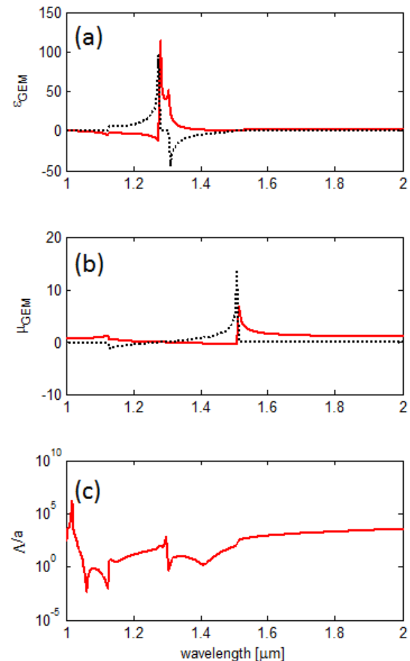
Figure 7. Effective \epsilon (a) and \mu (b) from GEM model for spheres of radius 0.2 \mu\text{m} , with \epsilon_2=12 in vacuum ( \epsilon_1=1 ) with a loading density of 25%, and the mean-free path (normalized to a ) for 1% vacancy density (c).
