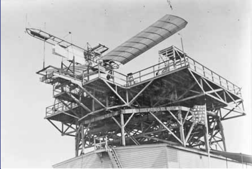
Samuel Langley's Aerodrome, December 8, 1903
