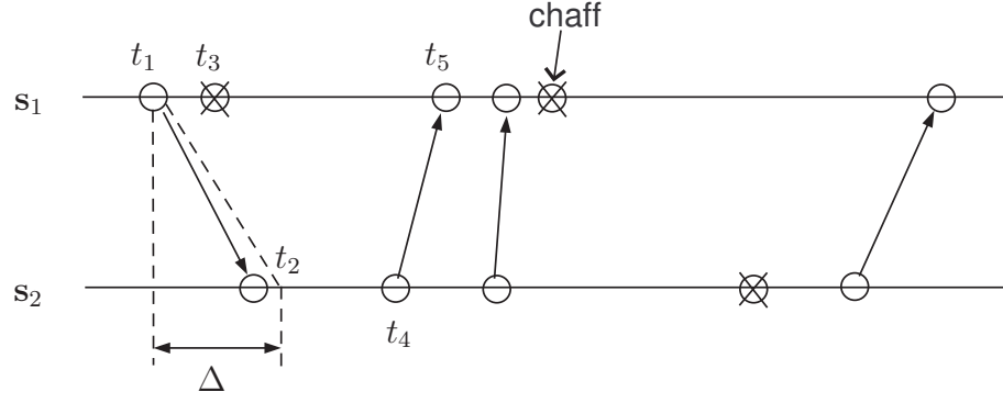
Figure 2.3: Bidirectional-Bounded-Greedy-Match
