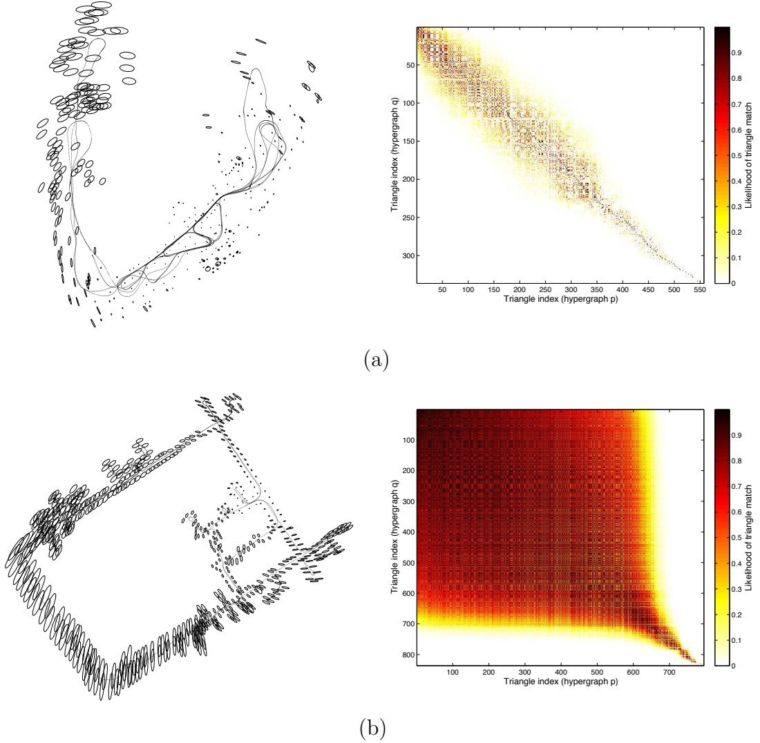
Figure 4.7: Data fusion and likelihood structure. An illustration of anisotropic data fusion in the coordinate system of a fusion agent p is shown above using the (a) Victoria Park and (b) DLR examples. The likelihood matrix \Delta in each case provides an indication of the underlying structure of the environment. In contrast to the likelihood matrix of the DLR environment, the matrix \Delta of the Victoria Park example naturally exhibits a banded structure.
