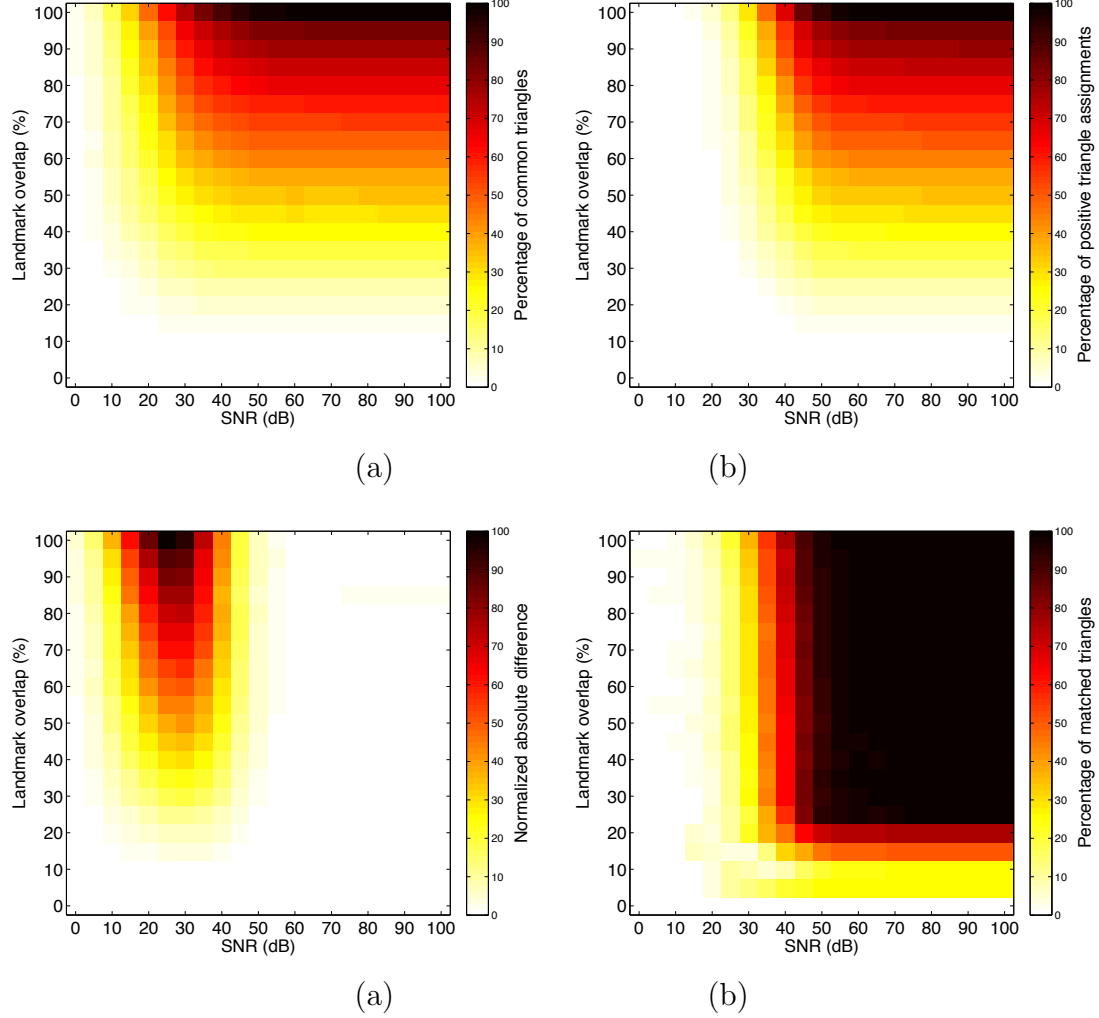
Figure 5.5: Monte Carlo performance of hypergraph matching. Varying the levels of noise and overlap results in a change in (a) the percentage actual common triangles relative to the ground truth of G_p and G_q and (b) the number of true positive common triangles determined by the linear assignment problem (LAP). The absolute difference between (a) and (b), normalized as a percentage, is shown in (c), which shows that the difference between the LAP solution and ground truth is small for a reasonably wide range of overlap and noise, resulting in the percentages of matched triangles after outlier rejection shown in (d).
