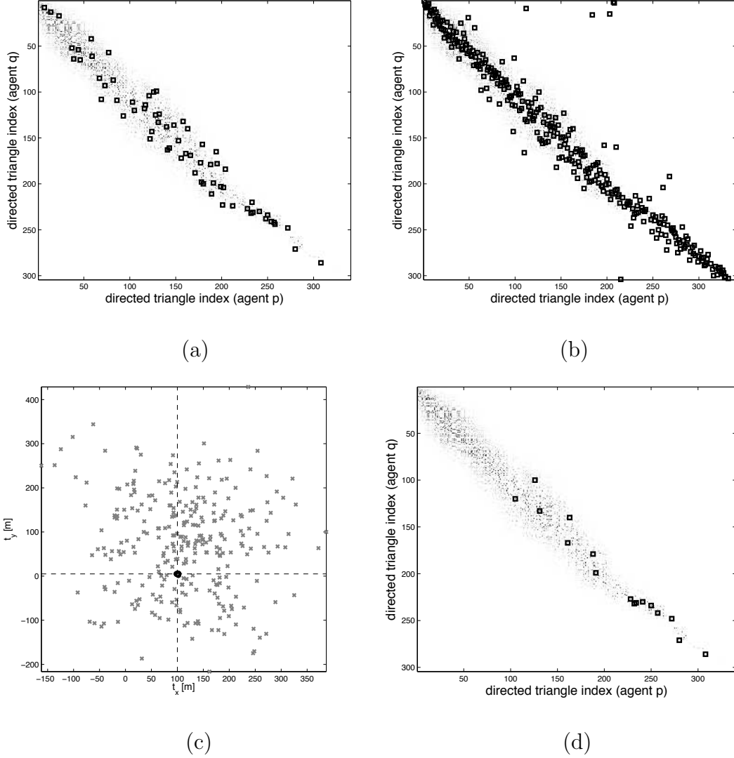
Figure 5.2: Hypergraph registration (Victoria Park example): likelihood statistics and outlier rejection. Markers are used to indicate entries of the likelihood matrix \Delta corresponding to (a) the true directed triangle matches, (b) the triangle matches specified by the linear program. (c) Inlier matches (black circles) are indicated by the rigid-body transform parameters that cluster around the true values of t and \theta , with outliers (gray crosses) indicated by the entries that fall outside the cluster. (d) After applying outlier rejection to the output of the linear program, 16 inlier matches are used to construct the registration solution \mathcal{R}^* .
