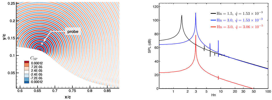
Figure 4: LES pressure contour of two-dimensional thermoacoustic waves generated from a sinusoidal heat flux input on the hump, where C_{SP} \equiv (p - p_\infty) / (\frac{1}{2} \rho_\infty a_\infty^2) , on the left. SPL is 112 dB at the probe location. Sound pressure spectrum of selected actuation Hn is on the right.
