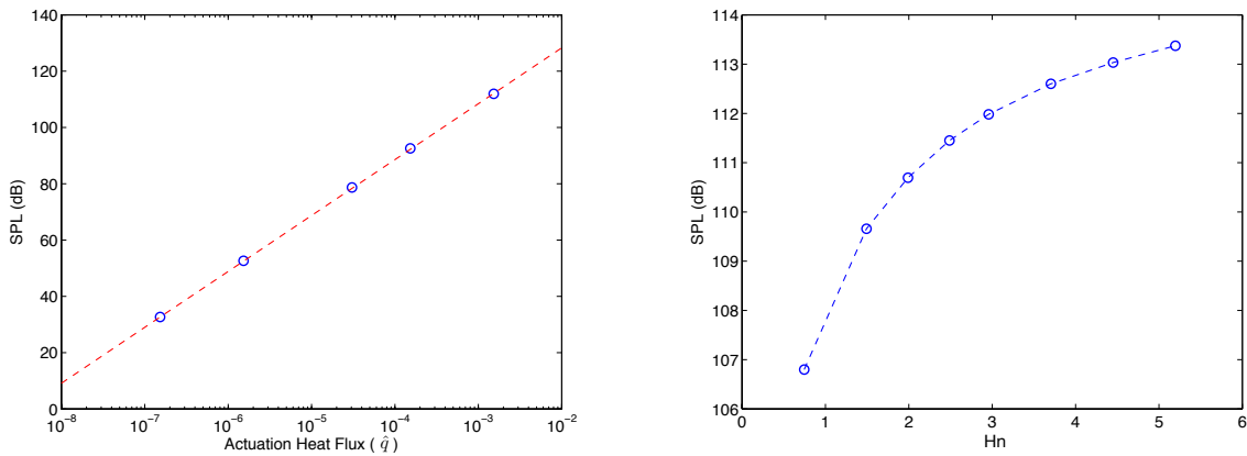
Figure 5: LES sound pressure at 5\sigma away (probe location) from the actuator. SPL at this point is plotted against the heat flux input, \hat{q} , on the left, and against actuation Helmholtz number, Hn, on the right.
