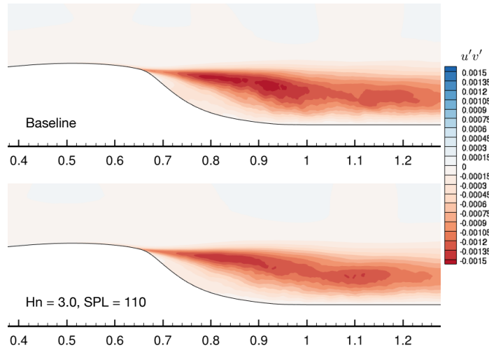
Figure 14: Spanwise Reynolds stress for three-dimensional simulation. The turbulent intensity is mitigated in the controlled case.
