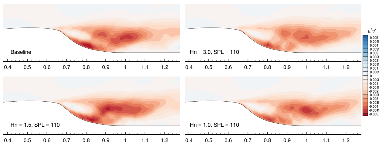
Figure 7: Spanwise Reynolds stress ( u'v' ) for the two-dimensional controlled flow in different actuation conditions.
