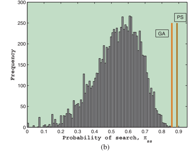
Figure 8. Monte-Carlo simulation for convergence and stability analysis and performance evaluation of Network#1. (a) Convergence and stability of genetic algorithm (GA). (b) Performance evaluation by Monte-Carlo simulation; GA= genetic algorithm, PS = pattern search.
