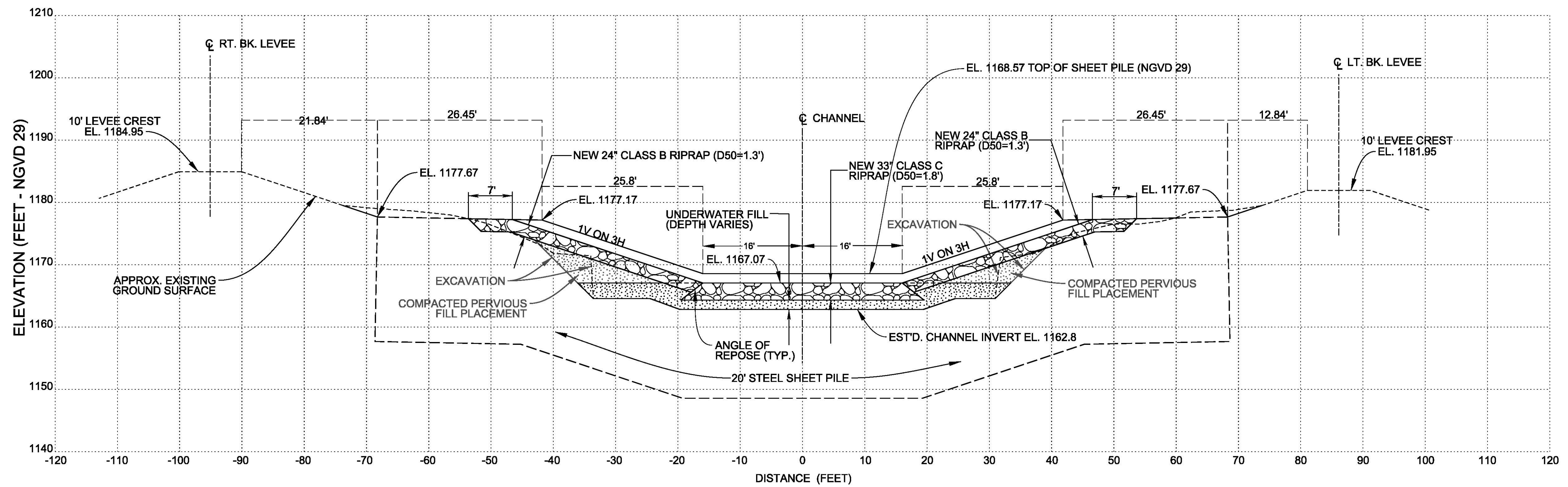
X-SECT. #1 - STA. 50+78.57C (LOOKING UPSTREAM) TYPICAL CHANNEL PROTECTION CROSS SECTION FOR STA. 50+68.57C - STA. 50+78.57C
