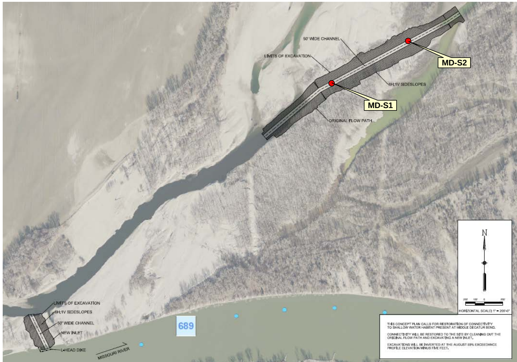
Figure 2. Proposed areas for excavation to restore connectivity at the Middle Decatur project site
