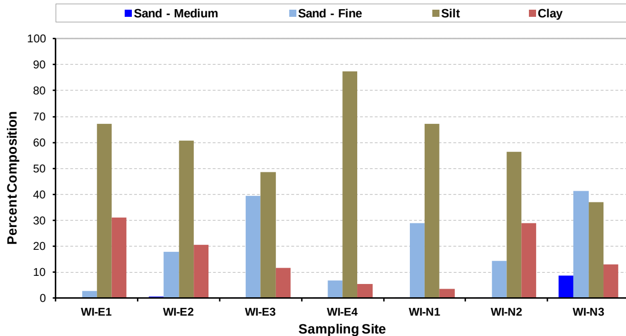
Figure 4. Particle size percent composition of sediment/soil samples collected at sites WI-E1, WI-E2, WI-E3, WI-E4, WI-N1, WI-N2, and WI-N3.
