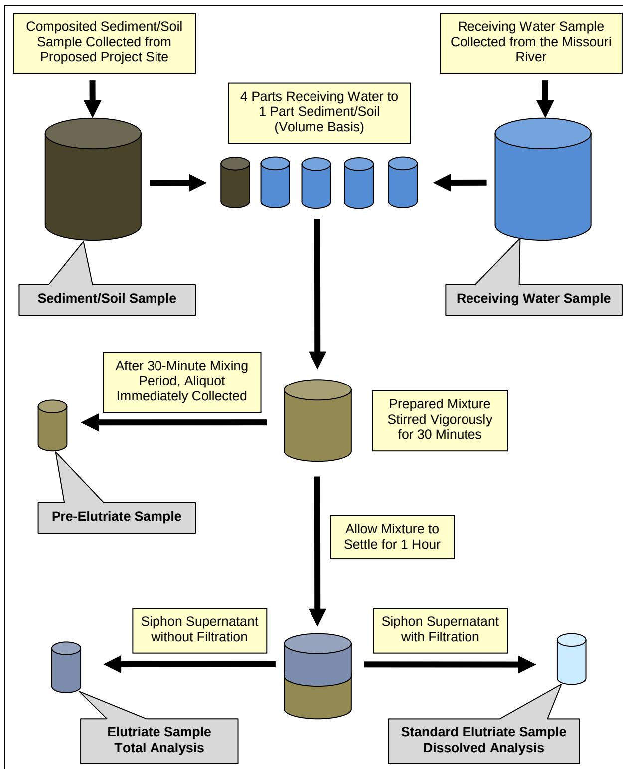
Figure 3. Process used to prepare samples for elutriate testing from sediment/soil samples collected at the proposed Wilson Island project site.
