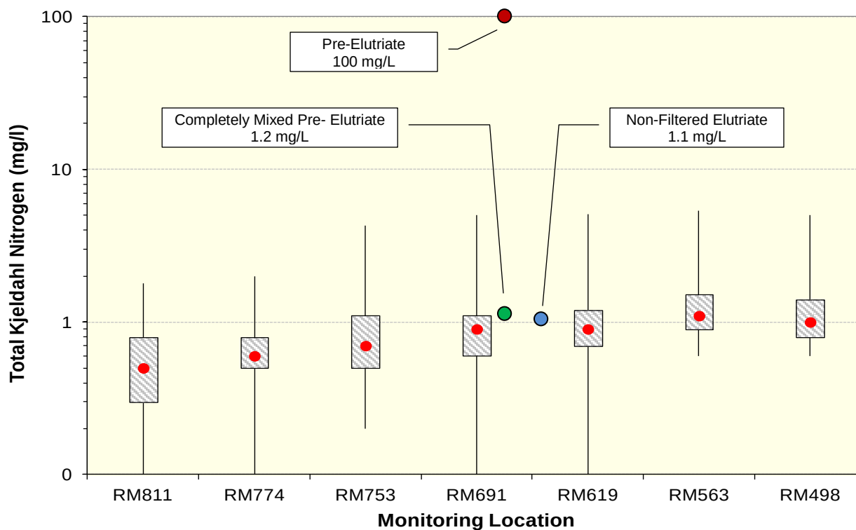
Figure 12. Mean elutriate testing results for Total Kjeldahl Nitrogen as compared to ambient Missouri River conditions monitored over the 5-year period 2007 through 2011.
