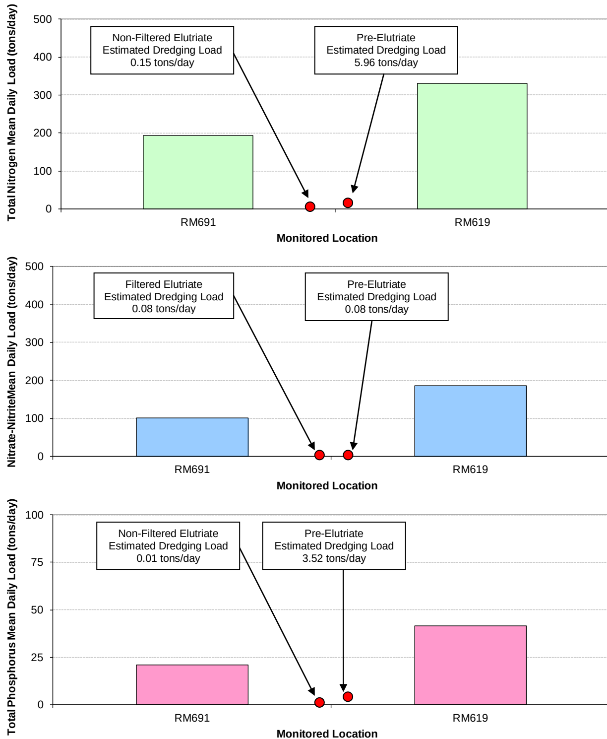
Figure 8. Comparison of estimated Total Nitrogen, Nitrate-Nitrite Nitrogen, and Total Phosphorus daily loadings from hydraulic dredging discharge to construct proposed shallow-water habitat at the Wilson Island project site to mean daily loadings calculated for the Missouri River at RM691 and RM619 over the 5-year period 2007 through 2011.
