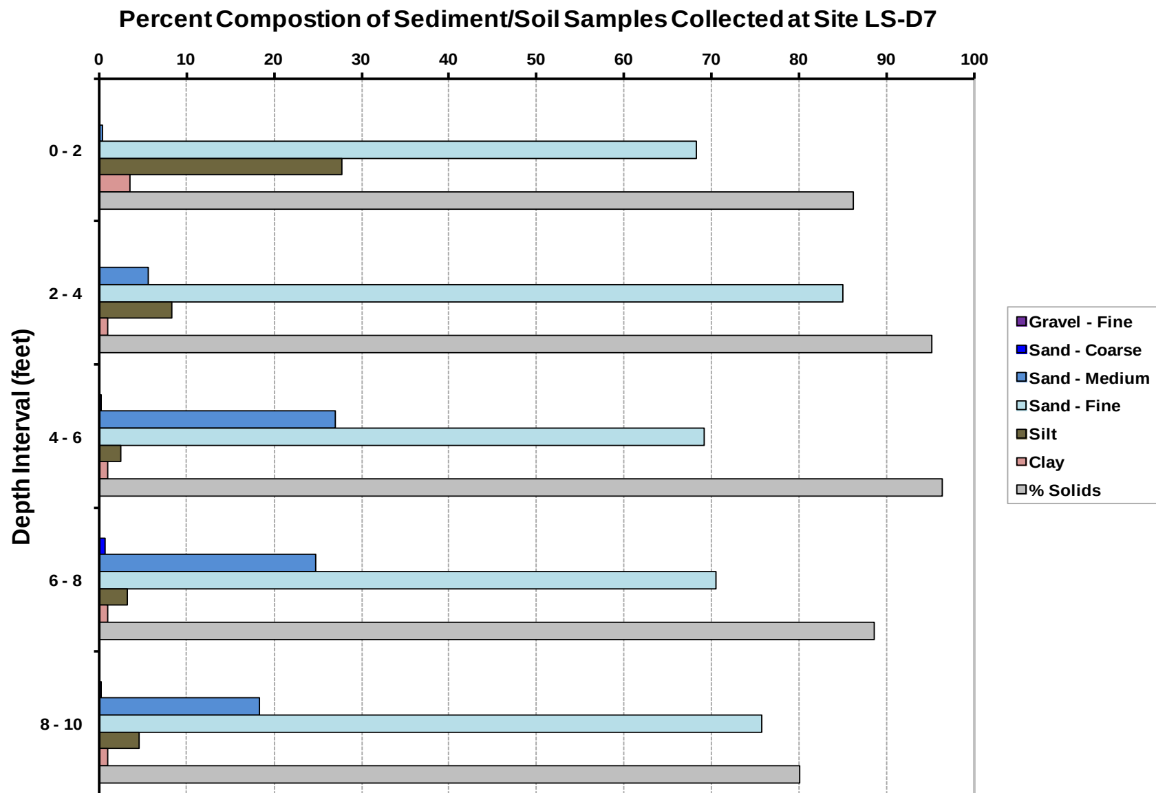
Figure 12. Percent particle size (dry wt.) and percent solids of depth-increment sediment/soil samples collected at site LS-D7.
