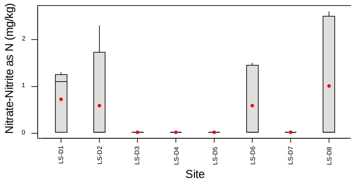
Figure 26. Boxplots of sediment/soil nitrate-nitrite as nitrogen levels measured at the eight sampling sites. [Note: The box represents the middle 50% of the data. The line through the box represents the median. The lines (whiskers) extending from the box represent the upper and lower 25% of the data excluding outliers. Outliers, if present, are represented by asterisks (*). The red point on each plot represents the mean.]
