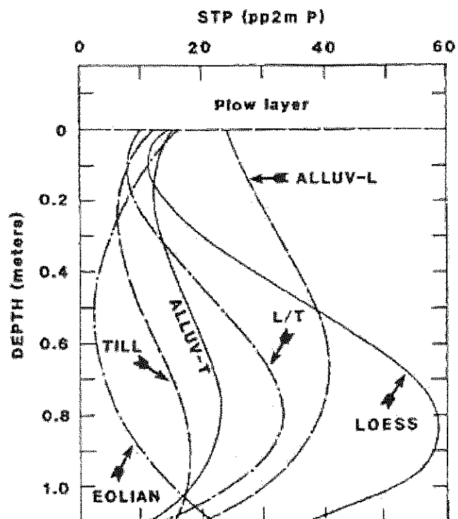
Figure 10. Predicted STP depth distribution for Iowa soil parent materials. From Kazemi, 1983.
