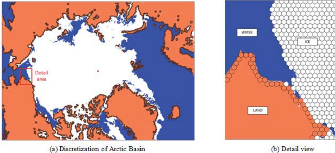
Figure 1. Demonstration DEM sea ice configuration initialization using the MASIE ice extent mask for July 1, 2014. There are two categories of polygonal elements in the DEM model: (1) Mobile ice floes (shown as white in (b)) and (2) immobile elements that represent the land mass boundaries (coral colored in (b)). This capability to initialize and discretize the sea ice cover using a raster mask is easily extended to any raster or vector polygon defined mask that delineates open water and ice.
