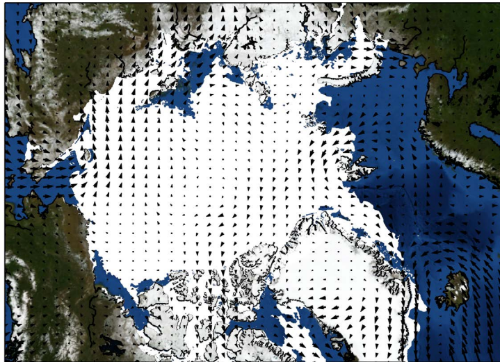
Figure 2. Wind forcing data (source: NAVGEM) overlaying the MASIE sea ice extent product for July 1, 2014. The weather forecast data will be used as the forcing for the DEM model sea ice dynamics. We are using output from several weather models to understand if the differences are sufficiently large to produce varying DEM model results.
