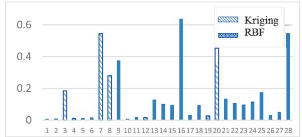
Figure 4: Max of Gradient of Response Surface.
