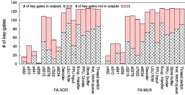
Fig. 11. Number of key-gates inserted at the outputs and inside the designs for different fault analysis-based insertion techniques.
