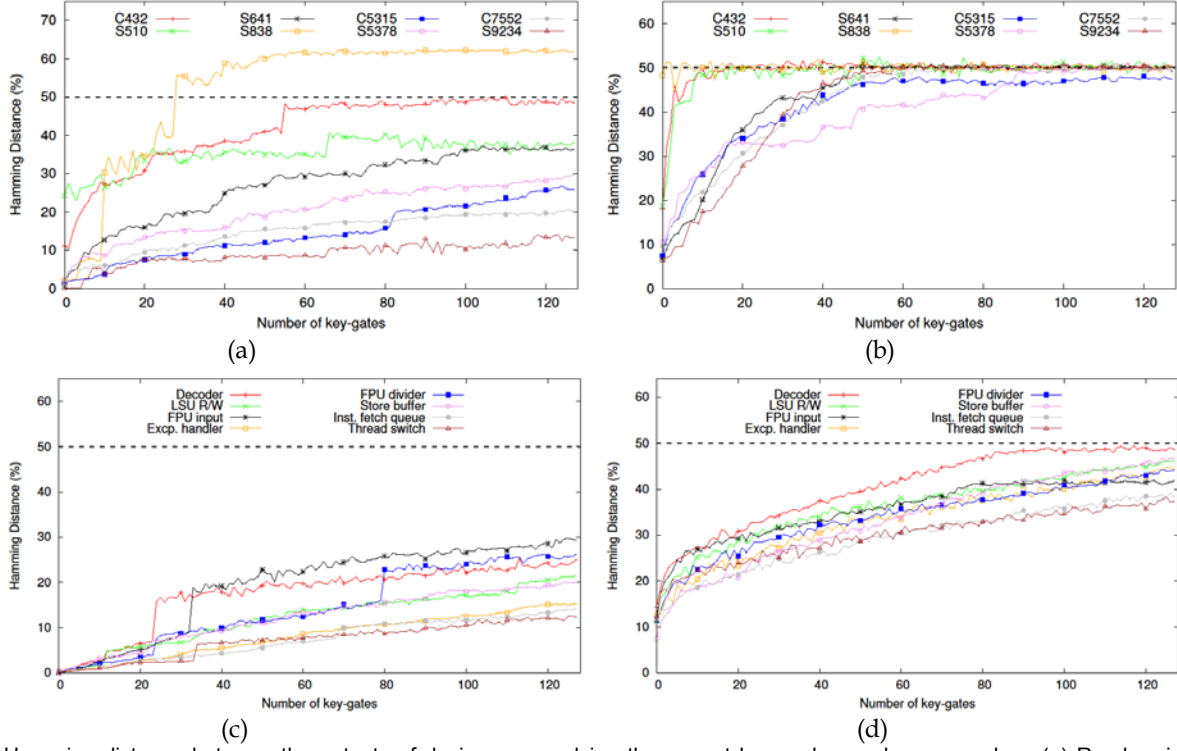
Fig. 7. Hamming distance between the outputs of designs on applying the correct key and a random wrong key: (a) Random insertion of XORs in ISCAS designs [6,7,11], (b) fault analysis-based insertion of XORs in ISCAS designs, (c) random insertion of XORs in OpenSPARC [6,7,11], and (d) fault analysis-based insertion of XORs in OpenSPARC units.
