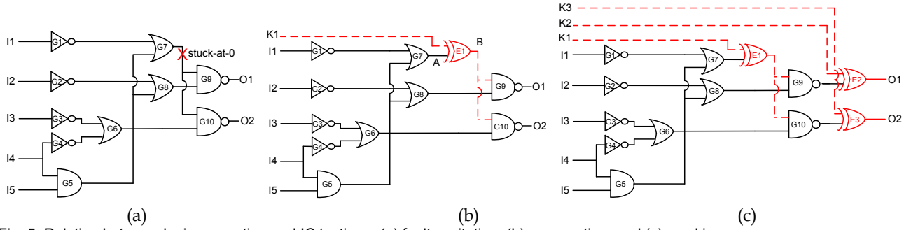
Fig. 5. Relation between logic encryption and IC testing – (a) fault excitation, (b) propagation, and (c) masking.
