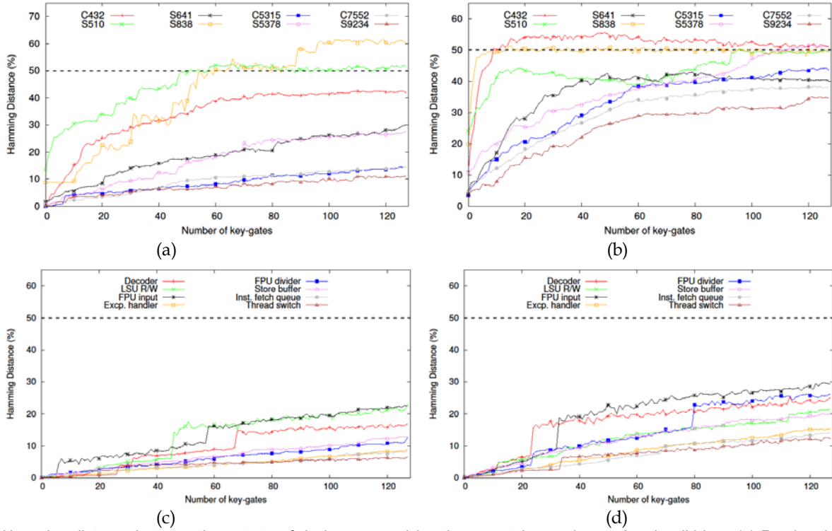
Fig. 8. Hamming distance between the outputs of designs on applying the correct key and a random invalid key: (a) Random insertion of MUXes in ISCAS designs, (b) fault analysis-based insertion of MUXes in ISCAS designs, (c) random insertion of MUXes in OpenSPARC units, and (d) fault analysis-based insertion of MUXes in OpenSPARC units.
