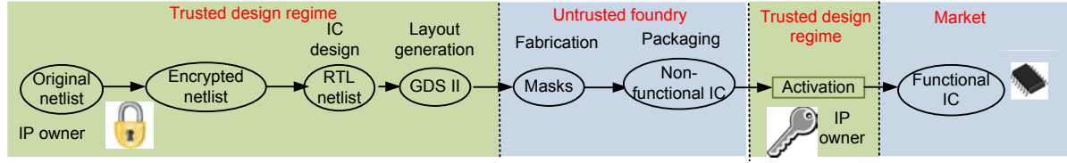
Fig. 1. An IC design flow enhanced with logic encryption capabilities to thwart IC piracy [6,7]. Before sending the design to an untrusted foundry, the designer encrypts the design using logic encryption techniques. The foundry then manufactures this encrypted design. On receiving the encrypted hardware, the IC designer activates it by applying the secret key and the IC is then sold in the market.
