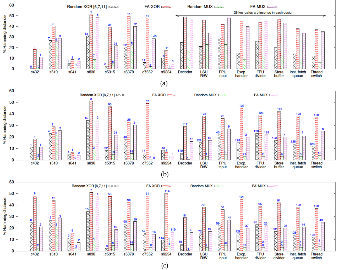
Fig. 10. Hamming distance achieved for different insertion mechanisms when the allowed overhead for logic encryption is 5%. (a) Power constrained, (b) delay constrained, and (c) area constrained. The numbers on top of the bar shows the number of key-gates inserted.
