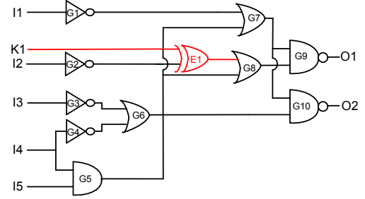
Fig. 4. A circuit encrypted with one XOR-gate (E1). The valid key is K1=0 . However, the design produces correct outputs ( HD = 0 ) for 24 inputs patterns out of the 32 possible input patterns.
