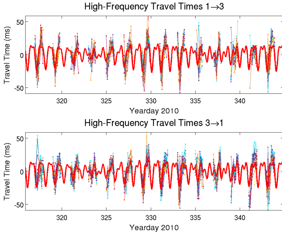
Figure Travel times obtained on reciprocal paths of the PhilSea'10 experiment compared to independent predictions. Only 30 days of a full year record length are shown. Some degree of non-reciprocity is indicated by this comparison. This 30-day record is indicative of the comparisons over the entire year record length, with occasional exceptions.
