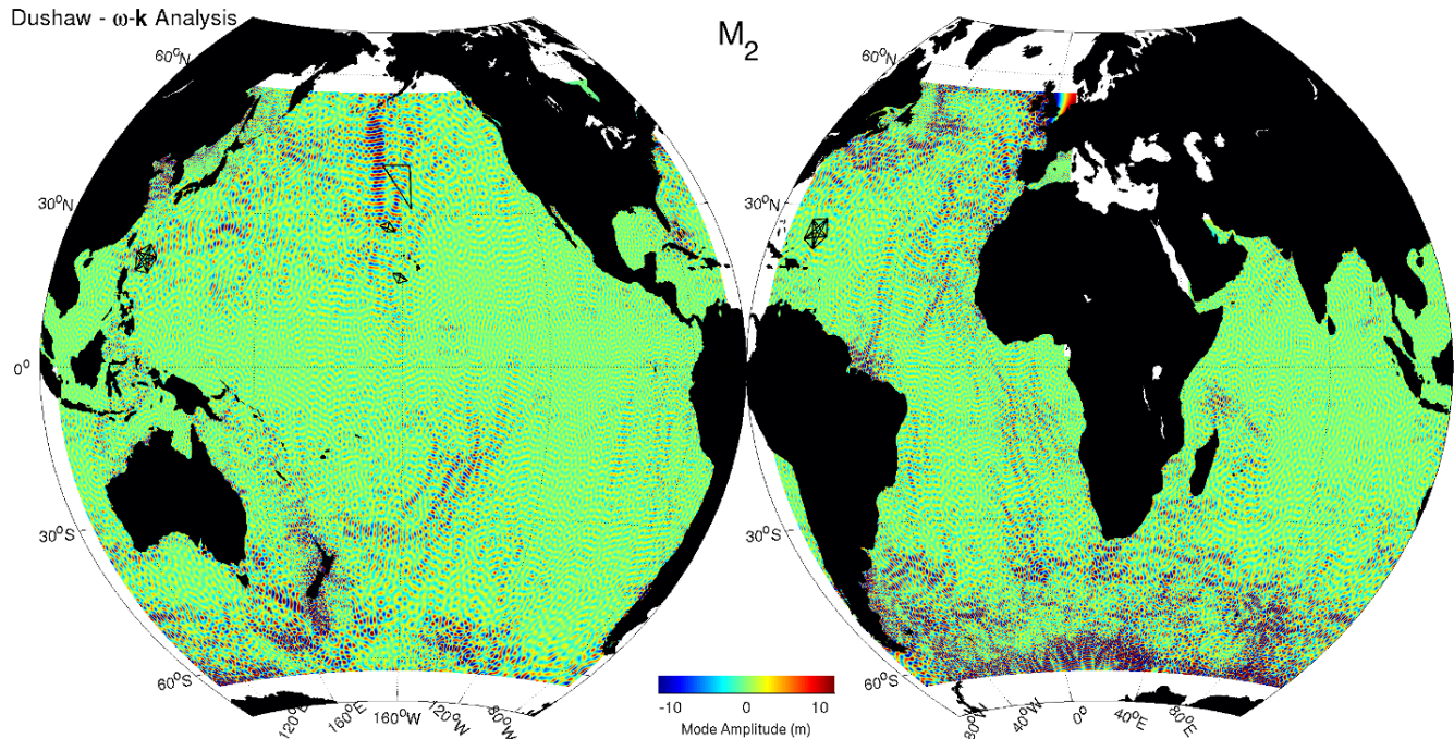
Figure Global estimates of the mode-1, M_2 internal tide amplitude derived from satellite altimetry following the frequency-wavenumber tidal analysis of Dushaw et al. (2011). These internal waves traverse ocean basins forming stable interference patterns. The mode-1 internal tide is predictable over most of the world's oceans. Tomographic observations of these waves were obtained using RTE'87 (central N. Pacific), AMODE (western N. Atlantic), HOME (Hawaii), and '09 and '10 Philippine Sea arrays, indicated. Agreement between tidal predictions from these maps and in situ observations is excellent.
