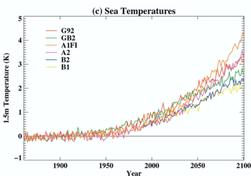
Figure 19. Time series of annual global mean sea temperatures in the 6 simulated scenarios for the period 1859-2100, each relative to their average over the period 1880-1920 (extracted from Johns et al 2003).
