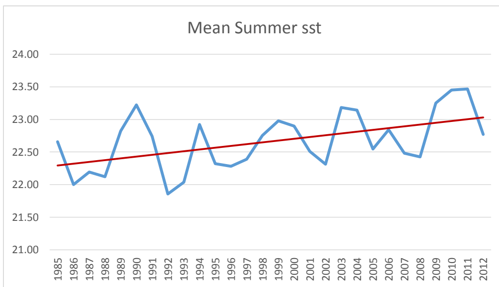
Figure 2. Climatology of annual summer sea surface temperature in the Alboran Sea
