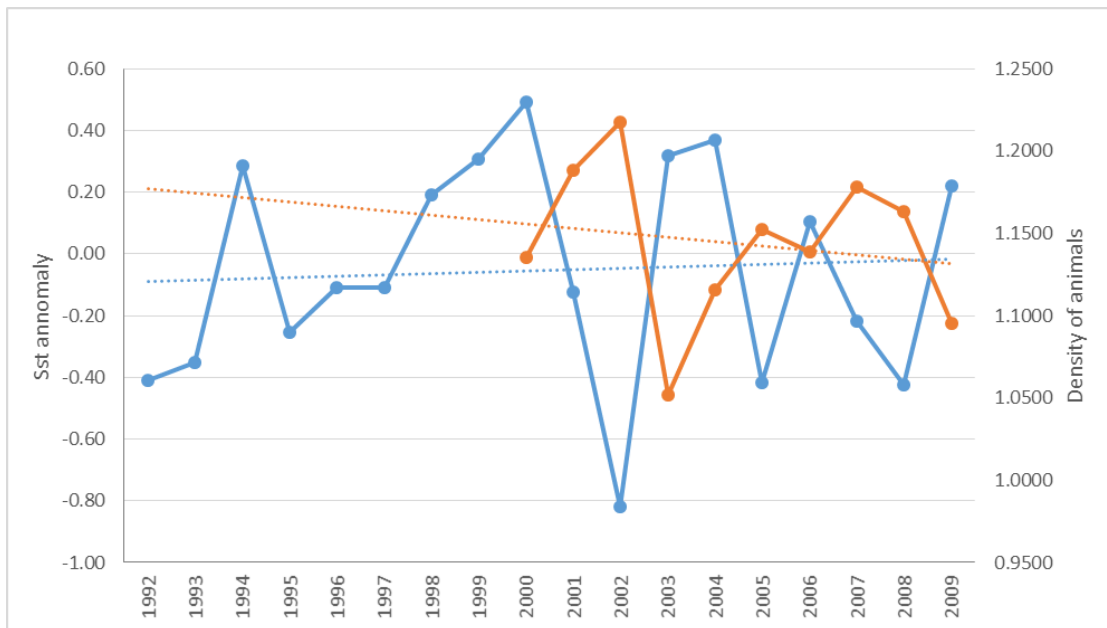
Figure 12. Plot of SST anomaly (blue) and density of animals (orange) in Alboran W from 1992 to 2009. Dash lines represent the linear regression lines for SST and density.
