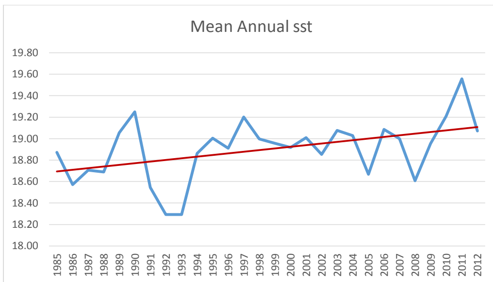
Figure 1. Climatology of annual sea surface temperature in the Alboran Sea
