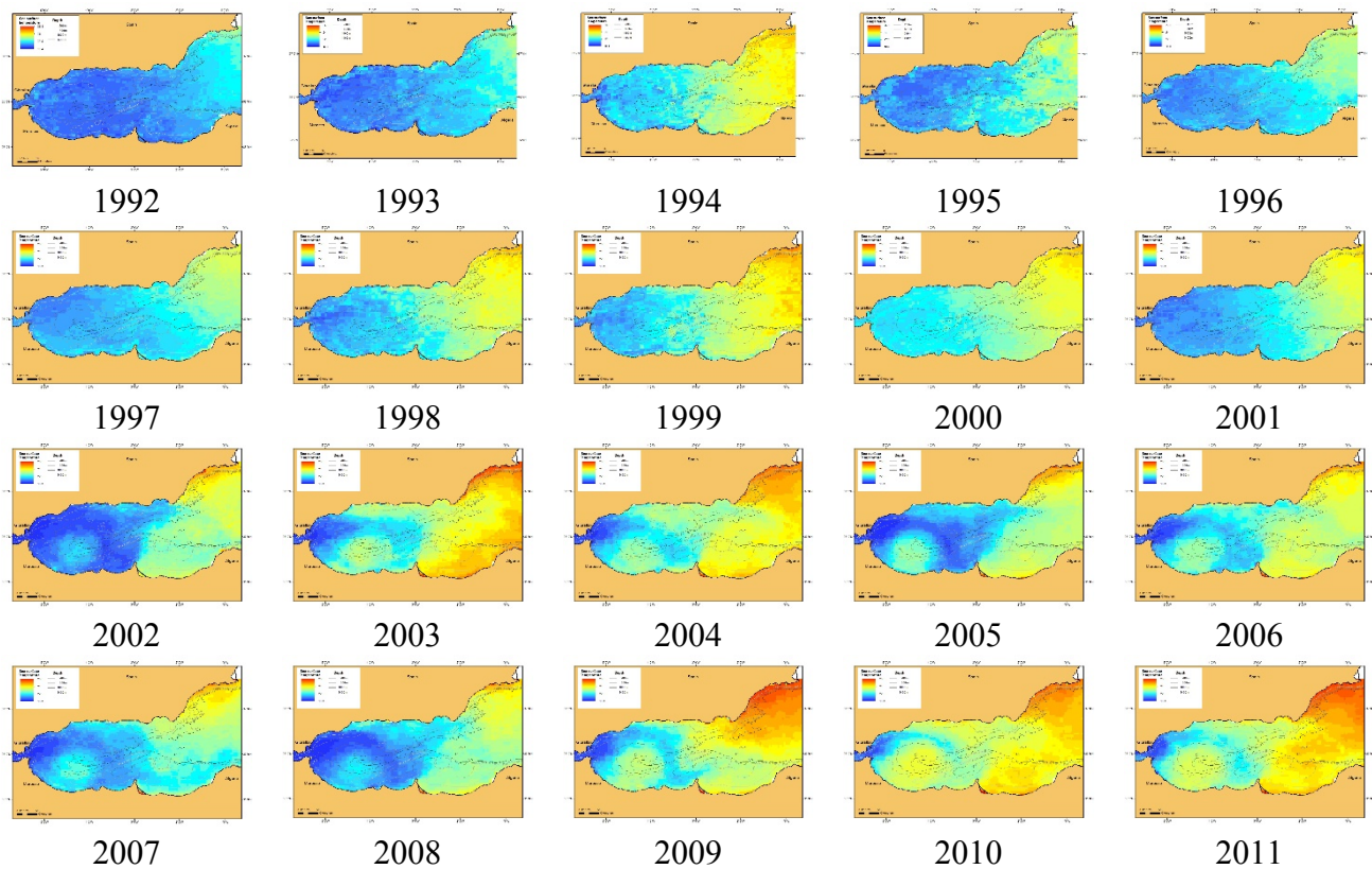
Figure 3. Sea surface temperature 1992-2011
