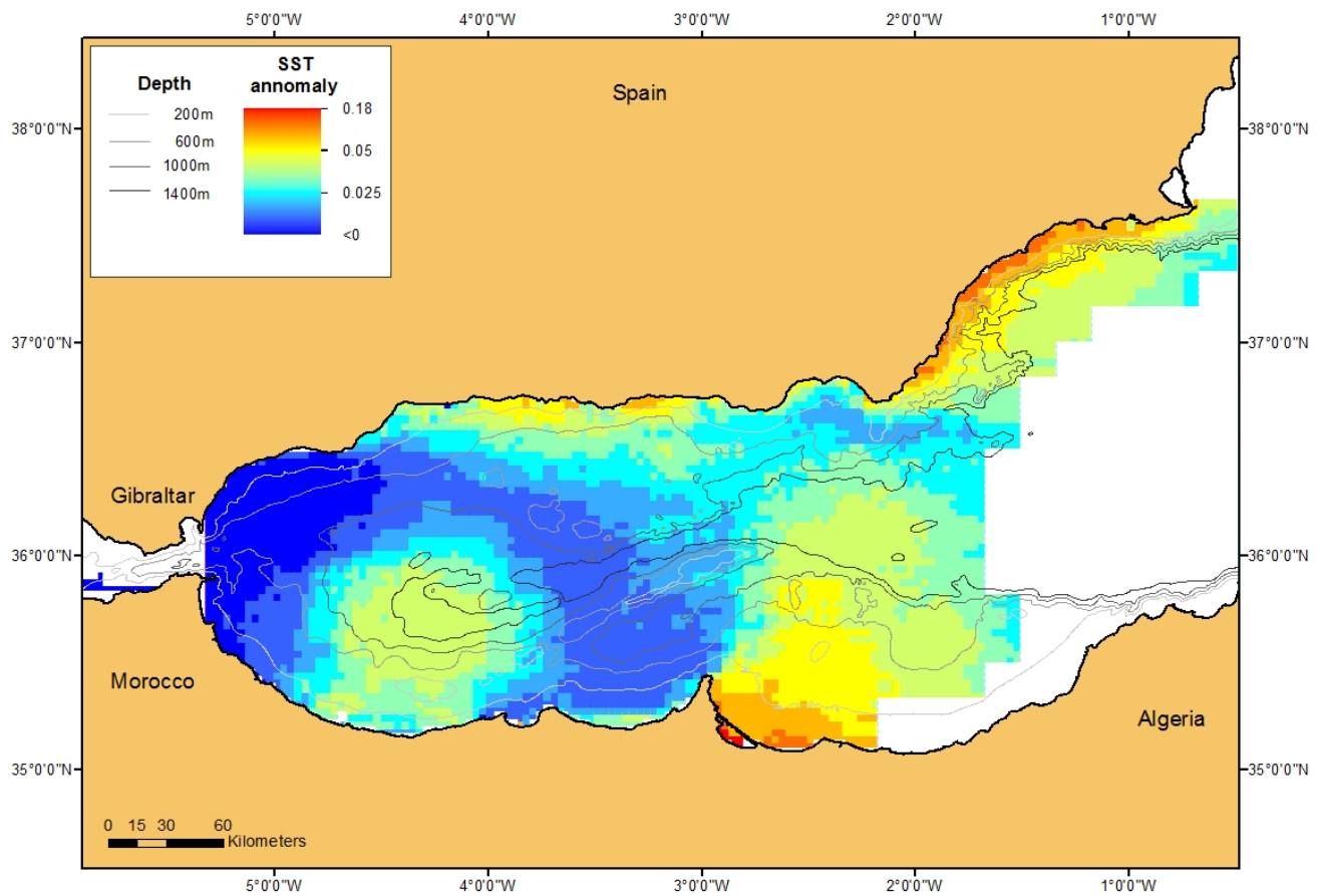
Figure 4. SST anomaly calculated for each grid cell.
