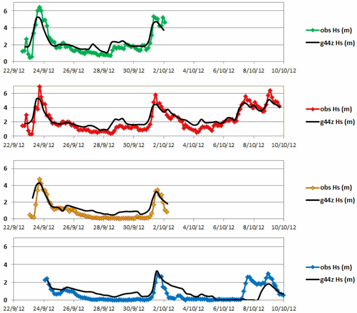
Figure 1: Significant wave height along the wave sensor drift trajectories as observed and from the model hindcast (black solid line).
