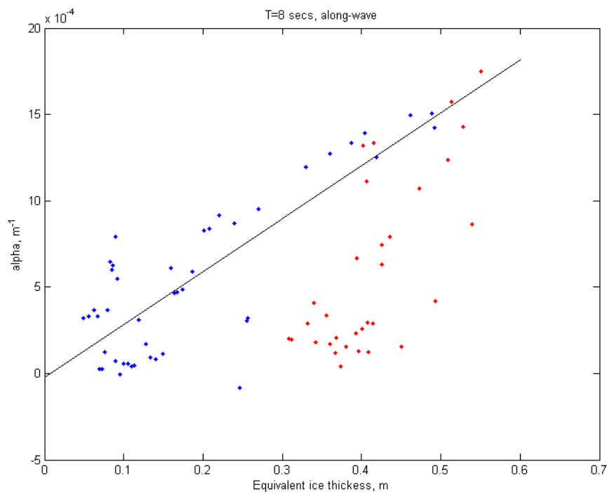
Figure 2: Dependence of wave attenuation on ice thickness, during the compression of the measuring buoy array (blue points). A linear dependence is clearly demonstrated.
