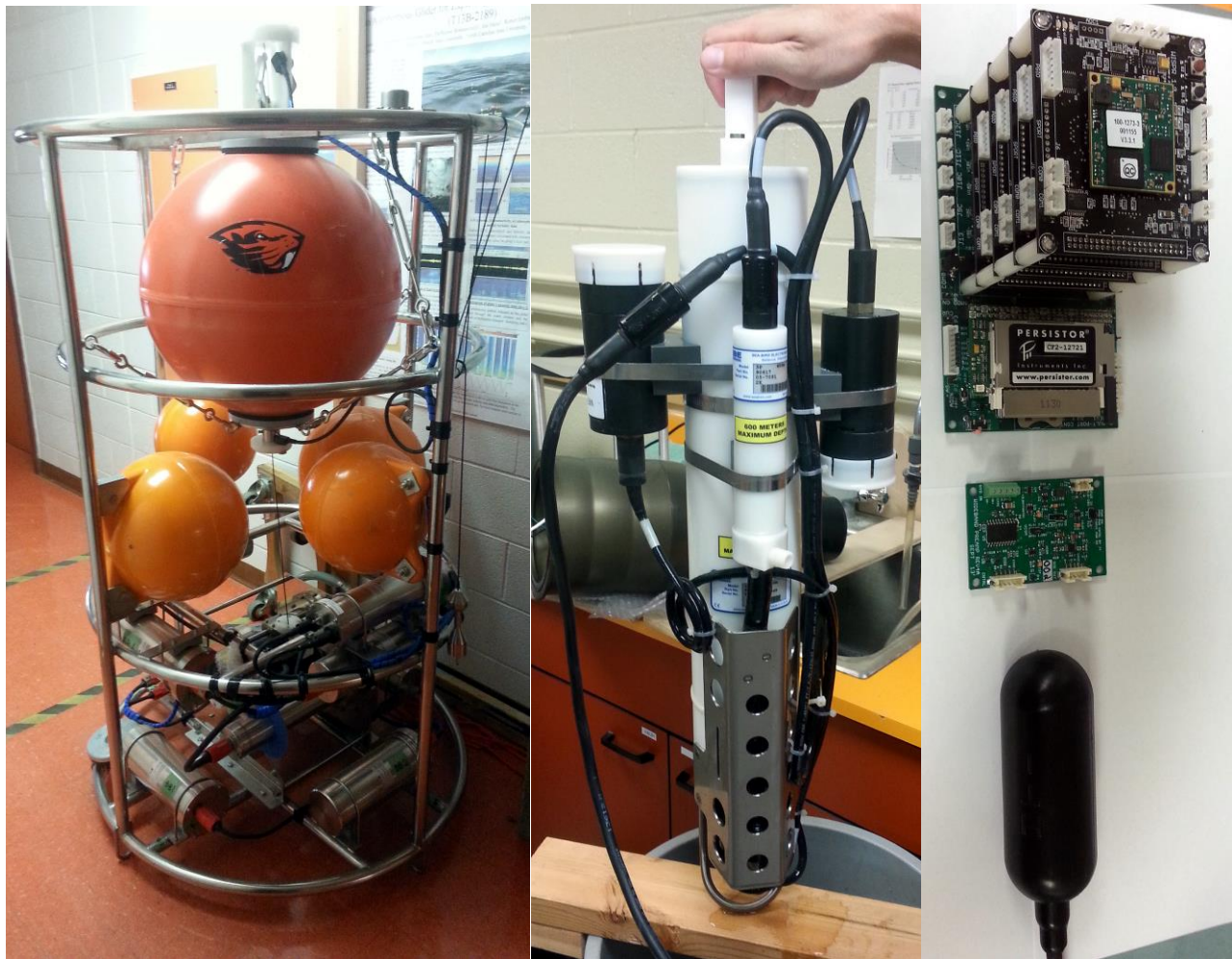
Fig. 2. Left: NGK underwater winch. Middle: Seabird CTD with PAR and Fluorometer sensor. Right: Multi-Port Controller incl. PAM.
