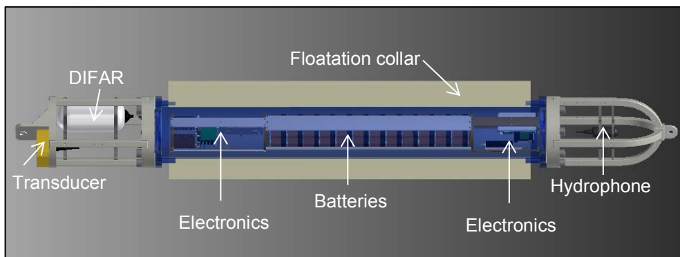
Fig. 3a: Mock-up of the sensor module.
