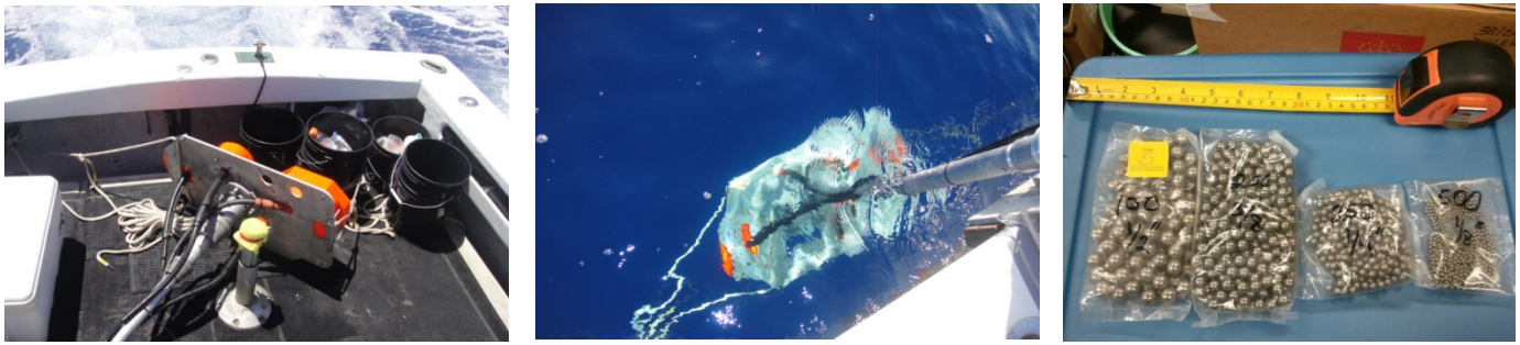
Figure 8. Multiple frequency echosounder array on boat deck (left) and in water (middle). Standard targets were steel spheres ranging in size from 3 to 25 mm (right).
