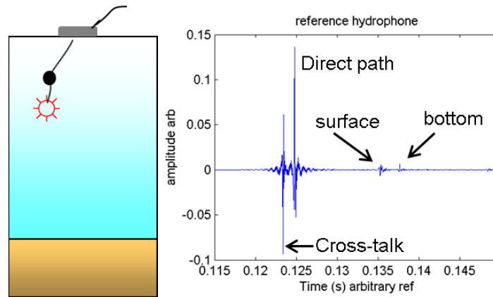
Figure 3 a) cartoon of normal incident seabed reflection experiment. The source (red) is nominally at a depth of 10.2 m and the receiver (●) is 2.17 m above the source. The source depth varied by \pm 0.5 m but is known to high precision being measured both by a pressure sensor and acoustically using time of flight to known boundaries (sea surface and bottom). The relative source-receiver distance had very small oscillatory excursions during the run of \pm 0.015 m. b) A typical example of the received signal showing the direct, surface, and bottom reflected paths.
