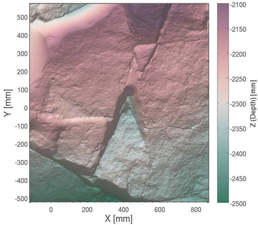
Figure 4. Estimates of high-resolution roughness taken near Larvik, Norway made with a stereo photogrammetry system.
