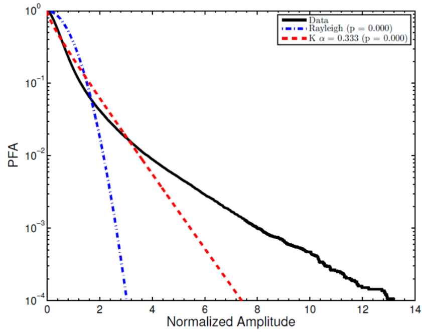
Figure 3. PFA of rock outcrop at 100 kHz obtained from FFI's HUGIN HISAS system.
