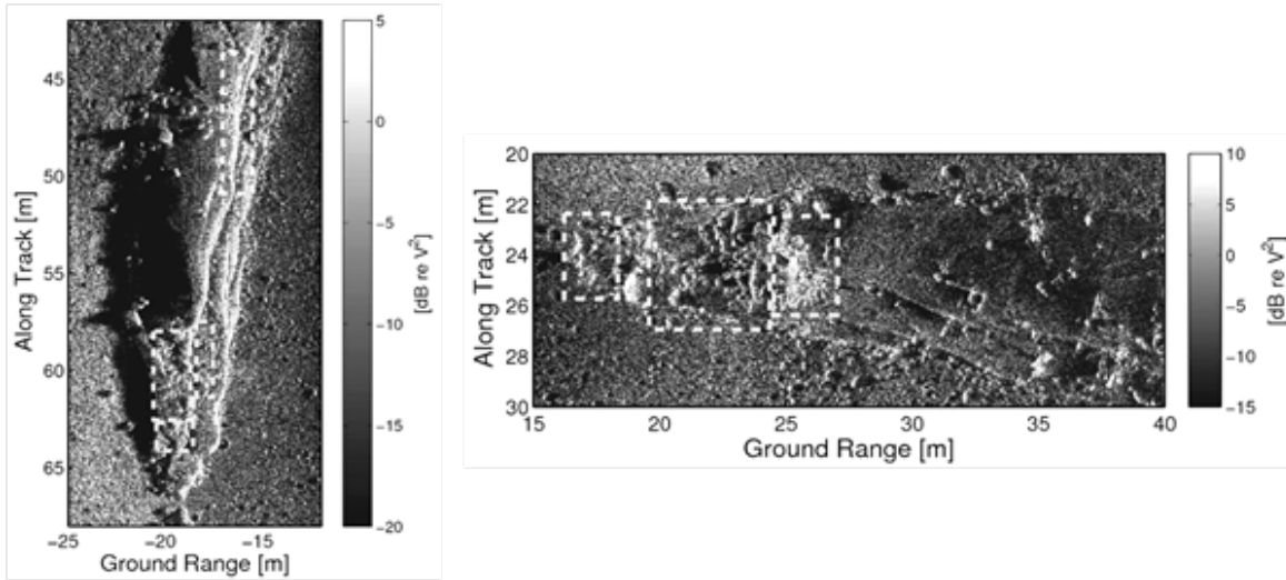
Figure 1. Synthetic aperture sonar images of a large rock outcrop in the Oslofford near Larvik, Norway, taken from two different look directions. Scattering strength was estimated for the areas outlined in the boxes and are shown in Figure 2.
