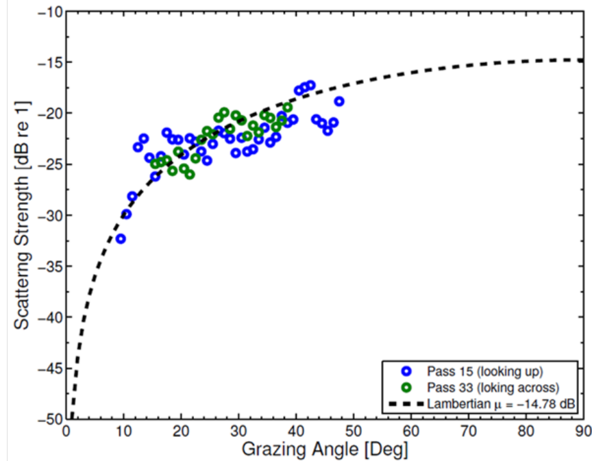
Figure 2. Scattering strength of rock outcrop at 100 kHz obtained from FFI’s HUGIN HISAS imaging sonar (circles) and a best Lambertian fit.
