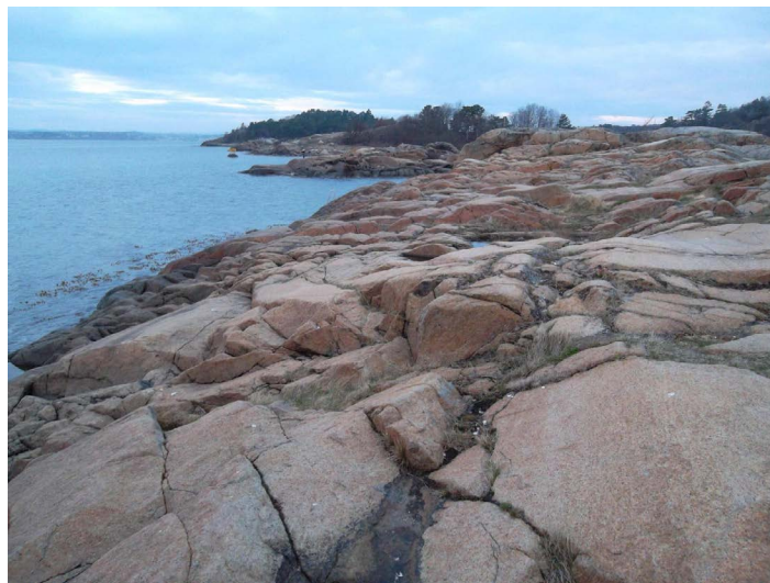
Figure 1. Photo of rock outcrop in the Oslofjord near Larvik, Norway. The outcrop is similar to underwater outcrops from which acoustic scattering was collected.
