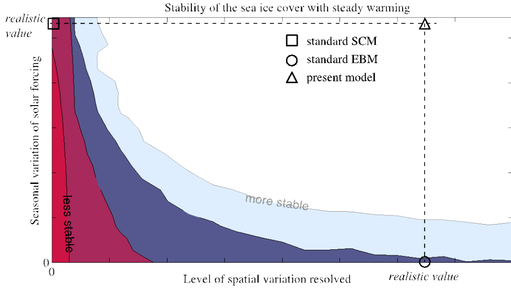
Figure 2: Dependence of the stability of the ice cover on horizontal diffusivity and seasonal variations. This is the result from 441 ~700-year simulations of warming and then cooling using the model described above.
