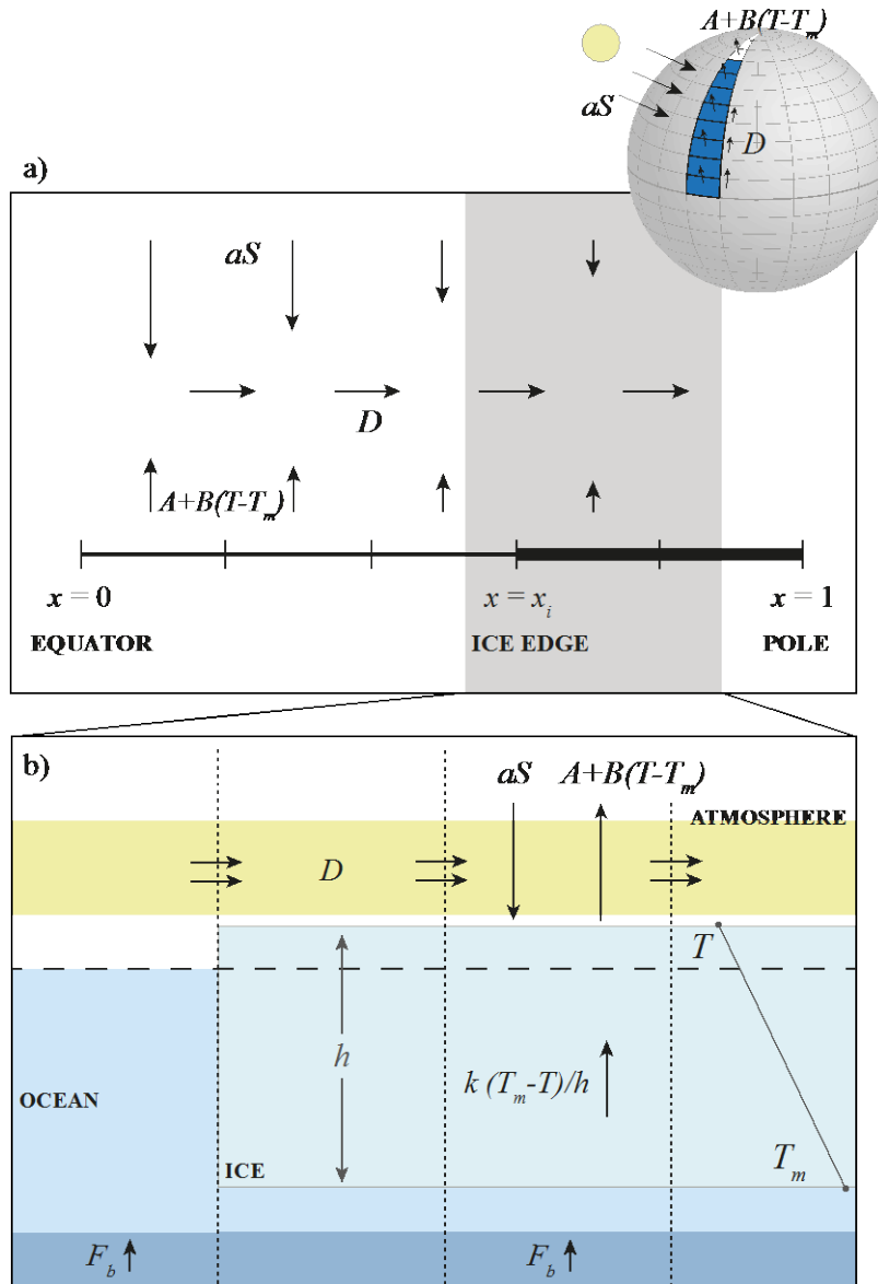
Figure 1: Schematic of the global sea ice and climate model developed under this project. Globe inset: Illustration of the model domain, a zonally-averaged aquaplanet. (a) Energy fluxes in the model atmosphere in the full model domain. (b) Energy fluxes in the model atmosphere, sea ice, and ocean in a subset of the model domain near the ice edge.
