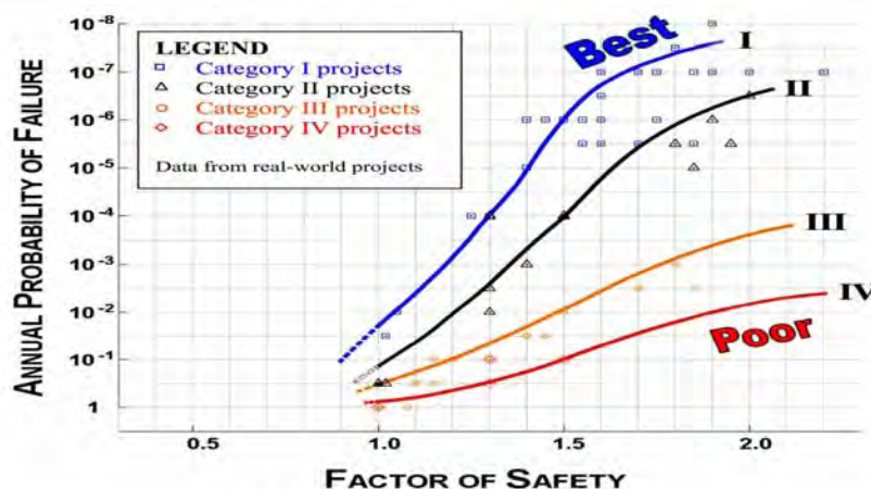
Fig. 1. Factor of safety versus annual probability of failure
