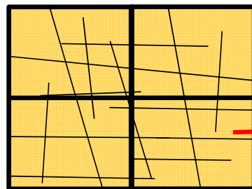
3-D spatial domain is discretized normally into volume elements
