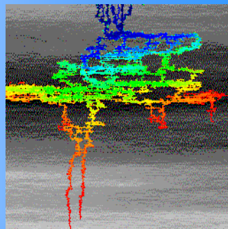
DNAPL Migration Ewing and Berkowitz, 1998
