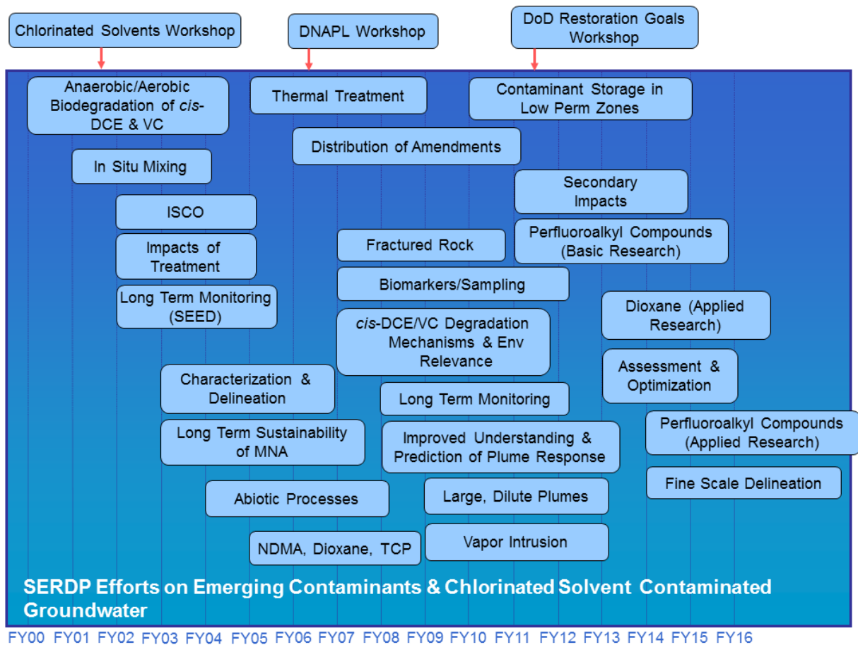
Figure 1 SERDP Efforts on Emerging Contaminants and Chlorinated Solvent Contaminated Groundwater
