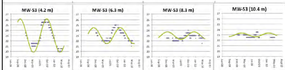
Figure 3: Measured and predicted groundwater temperatures. Blue diamonds show measured groundwater temperatures and green lines show predicted temperatures using model by Hillel, 1982. Model input values shown in this text.
