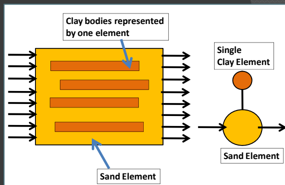
conceptual model mathematical model
