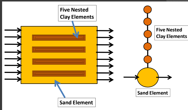
MINC conceptual model
