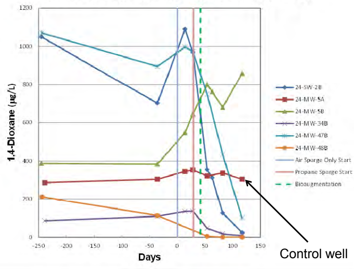
1,4-Dioxane Concentrations in the Demonstration Plot
