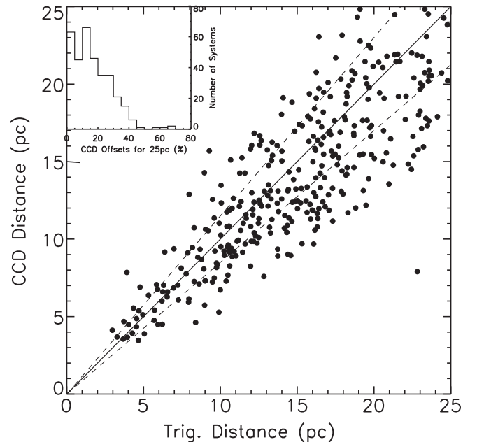
Figure 5. Distance comparisons of estimates from CCD photometry ( ccddist ) vs. distances measured using trigonometric parallaxes ( trgdist ) for the systems closer than 25 pc. Known unresolved multiples with blended photometry were not included. The diagonal line represents 1:1 correspondence in distances, while the dashed lines indicate the 15% errors associated with the CCD distance estimates. Note the reduced scatter compared to the similar pltdist plot shown in Figure 4, indicating the improvement in the photometry. The inset histogram indicates the distribution of the distance offsets between the pltdist and trgdist . For this sample, the absolute mean offset is 17%, consistent with the 15% systematic error determined by Henry et al. (2004).
