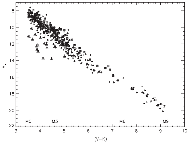
Figure 7. Observational HR diagram for all M dwarf systems in the sample that have trigonometric parallaxes and V magnitudes, using M_V and (V - K) as proxies for luminosity and temperature, respectively. Known multiples with blended photometry are enclosed in open squares. A set of a few dozen subdwarfs is evident below the main sequence. Spectroscopically confirmed subdwarfs have been enclosed in triangles, with references given in Table 3. Corresponding spectral type estimates are given along the bottom.
