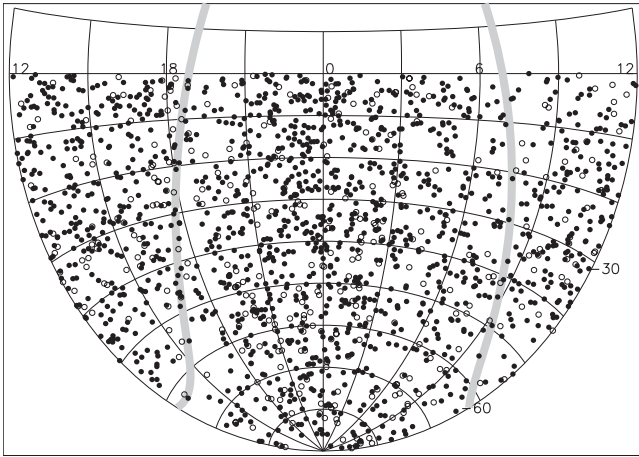
Figure 1. Distribution of the entire sample of 1748 M dwarf systems on the southern sky in R.A. and Decl.. Solid points indicate the 1404 systems within 25 pc, while open points indicate the 344 systems beyond 25 pc. The Galactic plane has been plotted in gray.
