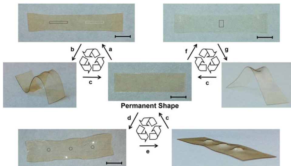
Figure 3. Shape-reprogramming. a) Room-temperature uniaxial hand stretching to \varepsilon = 33\% and then patterning with two 1.5 \mu\text{L} lines of 1 M NaOH (the black rectangle represents the top side and the white rectangle represents the bottom side). b) Heating of patterned film by hanging for 30 s at 120 ^{\circ}\text{C} . c) Soaking film in 1 M HCl for 20 min followed by heating for 1 min at 120 ^{\circ}\text{C} to recover the permanent shape. d) Room-temperature biaxial hand stretching to \varepsilon = 20\% in the x and y directions and then patterning with three 0.5 \mu\text{L} dots of 1 M NaOH (the pattern shown with black circles). e) Heating of patterned film in a PTFE dish for 5 min at 120 ^{\circ}\text{C} . f) Room-temperature uniaxial hand stretching to \varepsilon = 39\% followed by complete locking by soaking in 1 M NaOH for 1 h and then patterning with 5 \mu\text{L} of 1 M HCl. g) Heating of patterned film in a PTFE dish for 10 min at 150 ^{\circ}\text{C} . Scale bars: 0.5 cm.
