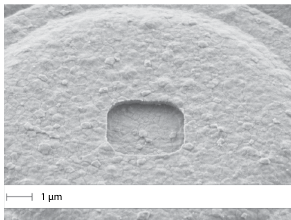
FIGURE 13 SEM image of polysilicon dome resonator. The poly2 shell is released by dissolving interpoly oxide through the irrigation hole (opening at the apex of the dome). The bottom polysilicon layer (poly1, visible through the irrigation hole) is covering a circular patch of field oxide conformally, defining the out-of-plane curvature of the dome.
