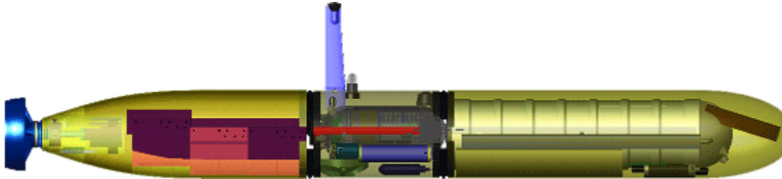
Figure 2. Bluefin 12 UUV
