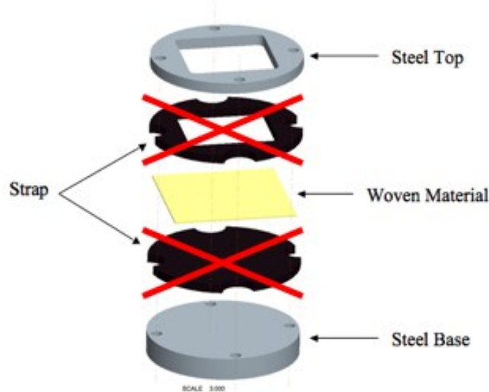
Figure 71: Revised clamping method without strap
