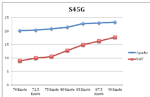
Figure 11. Shot from 45 degrees in Gorge (S45G), Closest Munition Distance
