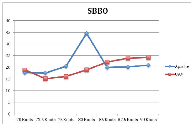
Figure 9. Shot from Behind and Below in the Open (SBBO), Closest Munition Distance
