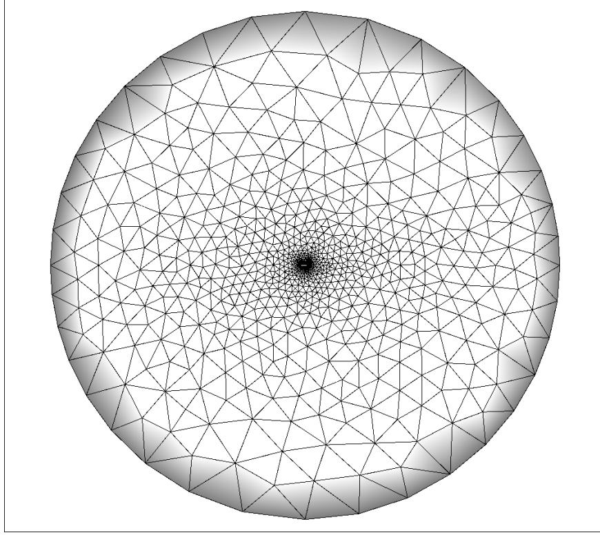
Figure 4.1: Airfoil grid
