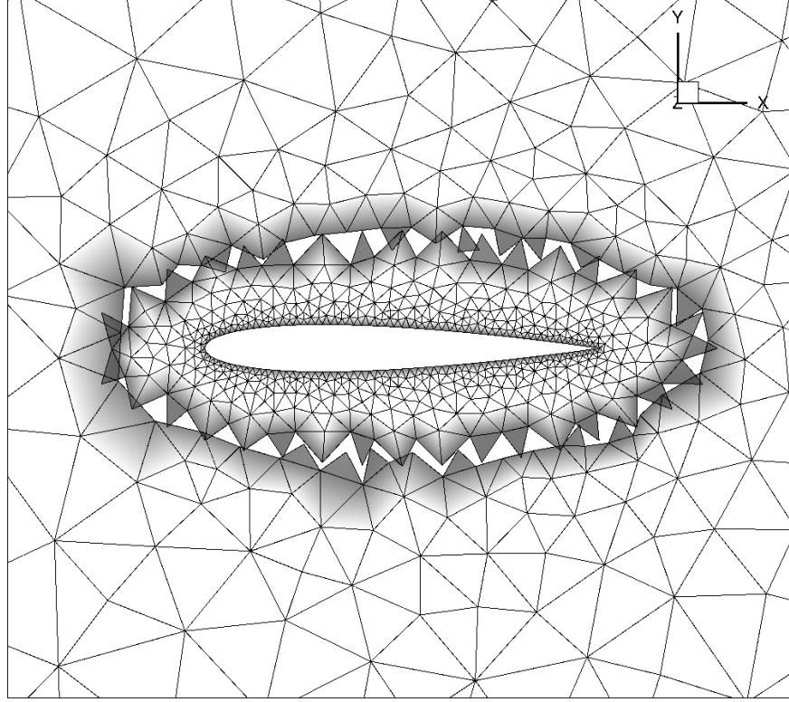
Figure 4.2: Overset grids
