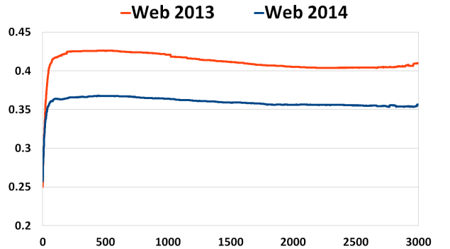
Figure 1: The learning curve of ListNet in the first 3000 iterations, with learning rate set to 0.01. The X-axis is the number of iterations for the training of the 1-layer neural network (NN), the Y-axis is the optimization criterion correlated to MAP. The features were collected based on the full ClueWeb12 dataset.
