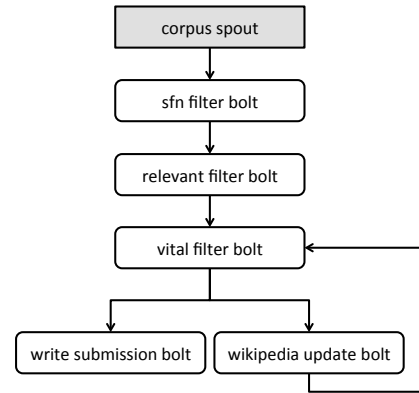
Fig. 1. Topology of our system developed on Storm.
