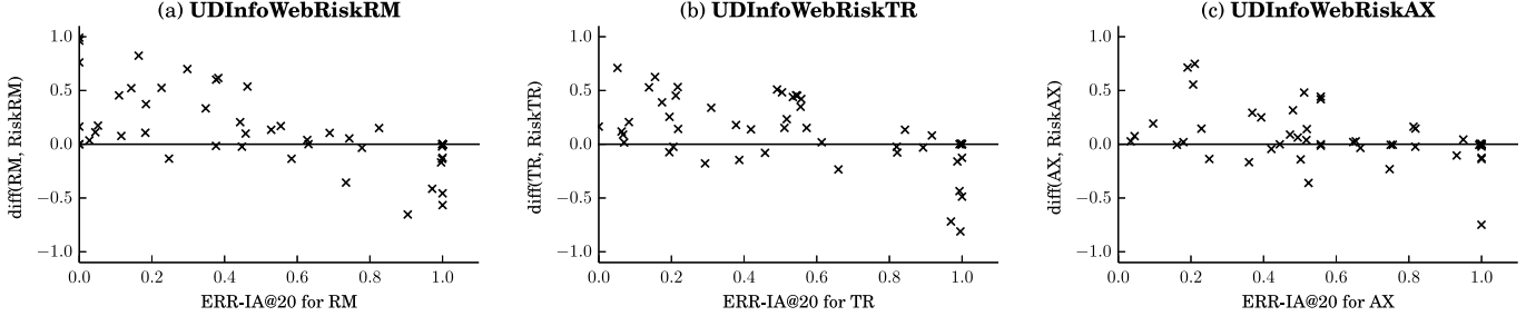
Figure 2: Impacts of latent entity space model on different baselines (ERR-IA@20).
