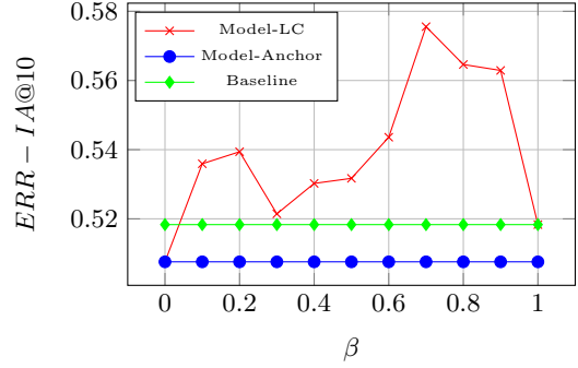
Figure 5: Impact of fusion weight ( \beta ) on ERR-IA@10 .
