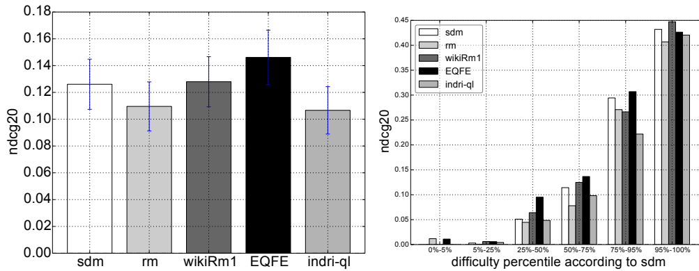
(a) Mean retrieval effectiveness with standard error bars (b) Mean retrieval effectiveness across different query-difficulties, measured according to the percentile of the SDM method.
