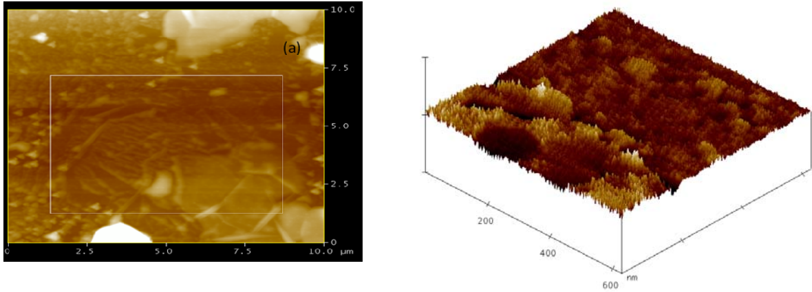
Fig. 17: AFM image of graphene (a) transferred to quartz substrate, (b) 10 layer \text{Fe}_3\text{O}_4 patterned on graphene.
