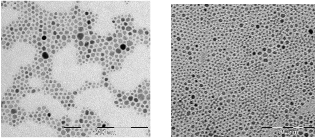
Fig. 12(a): TEM image of as synthesized \text{CoFe}_2\text{O}_4 nanoparticles. 12(b): Particles dispersed in Rogers polymer showing excellent dispersion
