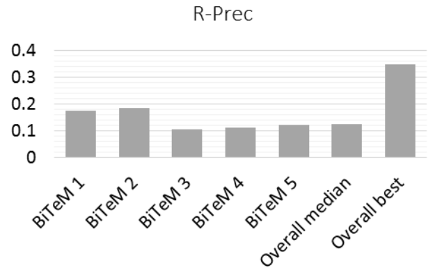
Figure 2. Different official R-Prec values, for the BiTeM runs and the other teams' runs (median and best).
