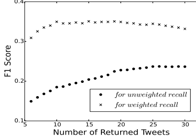
Figure 2: F1 Score Increases When Returning More Tweets for UDInfoMMRWCA run
