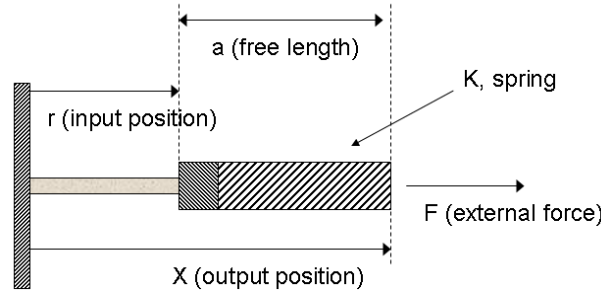
Figure 2. In a robotic tendon model, the motor turns moving a nut inward or outward adjusting, r . The external force, F , and position, x , describe the desired outputs. A spring is placed in between the nut and the external force. The free length of the spring is given by, a .
