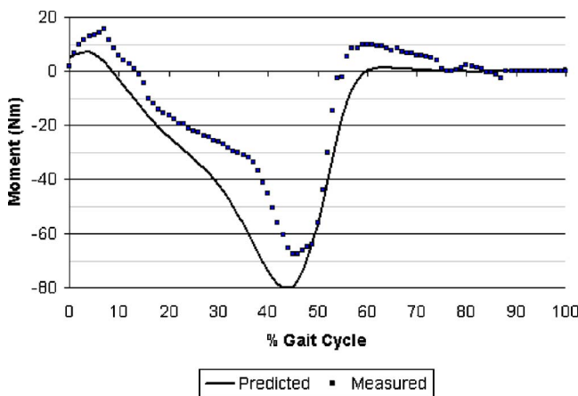
Fig. 6 The predicted moment is calculated from Fig. 2. The measured moment is calculated knowing the deflection of the spring during the gait cycle.
