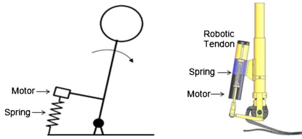
Fig. 1 Desired spring deflection is achieved by controlling the motor position and capitalizing on the cyclical nature of gait. As the tibia rotates over the stance foot, springs are extended. Simultaneously, the motor extends the springs to achieve the desired spring deflection and the forces required to generate the required ankle moment for walking. This inverted pendulum with a lumped mass illustrates the regeneration energy with use of a spring in series with a motor. Computer aided design model of the prototype is illustrated on the right.
