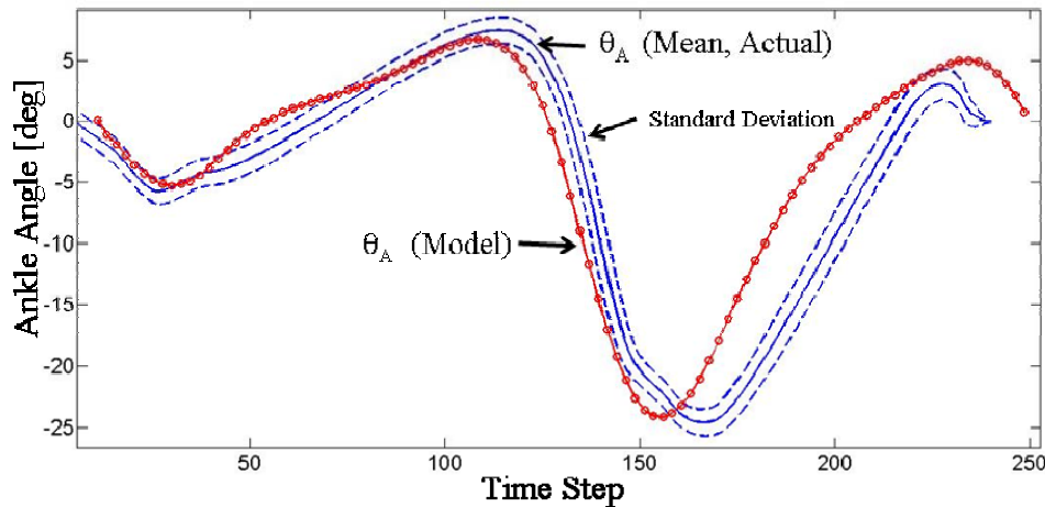
Figure 8: The subject walks on a treadmill at 2.2 mph. The ankle has 9 degrees of dorsiflexion and more importantly 23 degrees of plantarflexion based on the actual lever displacement. The user has complete control of the ankle motion because the output side of the spring is not controlled. The actual lever displacement fits the model extremely well.
