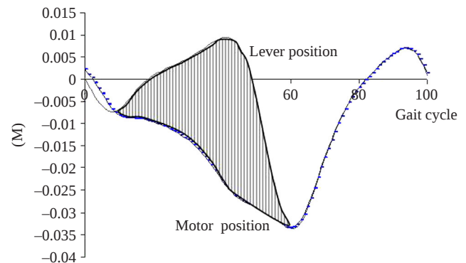
Figure 2 Desired spring deflection, shaded area, is achieved by controlling the motor position and capitalizing on the cyclical nature of gait
