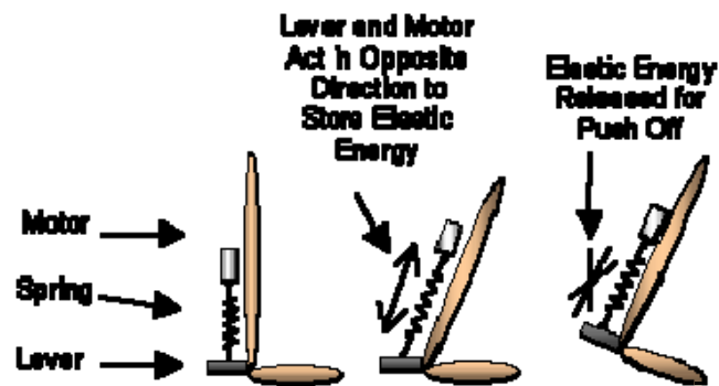
Figure 4: In our prosthetic ankle, the motor and spring are mounted behind the leg. We use springs to store and release the needed energy. As the leg rolls over the ankle, the motor attached to the proximal side of the spring and the lever attached to the keel and the distal side of the spring both pull on the spring in opposite directions. The stored energy is then released for powered plantarflexion.
