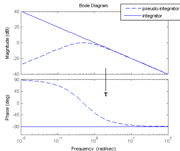
Fig. 9. Bode plot of the pseudo-integrating transfer function along with an integrator.
