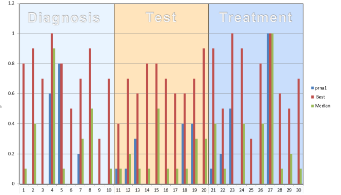
Figure 4: Prec(10) scores for each topic
