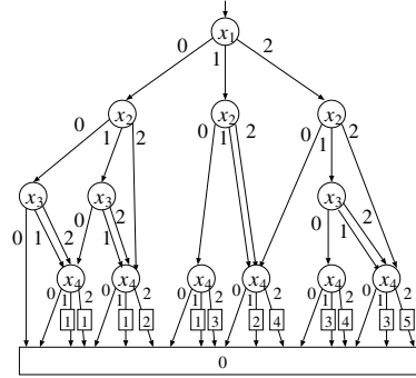
Figure 3. EVMDD for the structure function [11].
