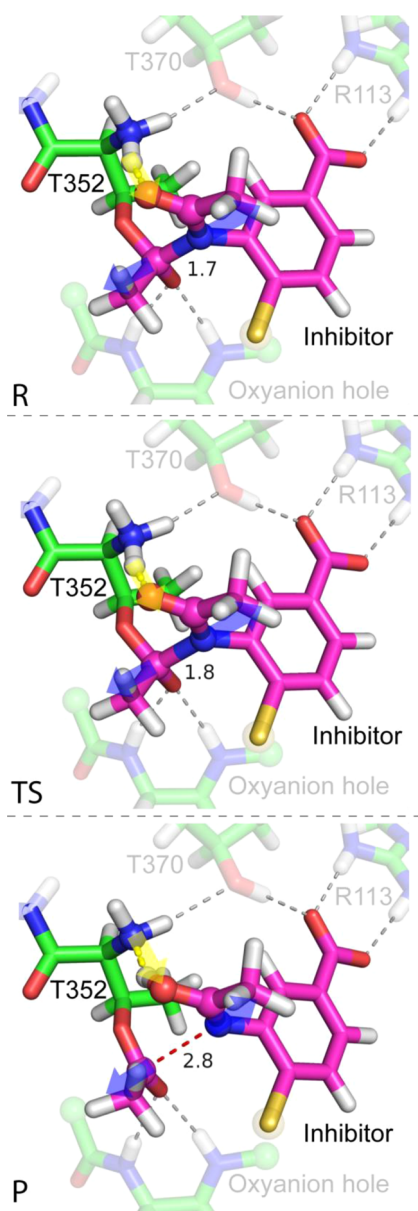
Figure 11. Reactant, transition state, and product for the formation of the acetylated CapD and iminol leaving group of capsidin. Snapshots of the QM region of the ONIOM(QM/MM) system along the reaction path. Enzyme carbon atoms are colored green, whereas inhibitor carbon atoms are colored magenta. Hydrogen, nitrogen, oxygen, and sulfur atoms are colored white, blue, red, and yellow, respectively. Hydrogen bonds between the ligands and the enzyme are shown as dashed gray lines. Dashed yellow lines connect the atoms that are involved in the chemical transformations. The residues of the active site that are not directly involved in the reaction are shown in faded, transparent colors. Atoms that link the QM region to the rest of the system described by molecular mechanics are depicted with transparent spheres around them. These atoms are substituted for hydrogen atoms, and their bond lengths are adjusted accordingly during QM calculations. The direction of the proton transfer is shown with a yellow transparent arrow. The coupled breaking of the scissile bond is shown with blue transparent arrows.
