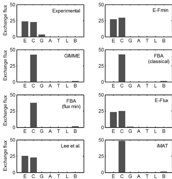
Figure 3. Exometabolome data of Saccharomyces cerevisiae and model predictions. Bars represent experimental and predicted values of exchange fluxes when the glucose uptake was A 16.5 and B 11.0 mmol/(gDW·h). Capital letters on the x-axis denote the production rates of extracellular metabolites, i.e., E: ethanol production, C: CO 2 production, G: glycerol production, A: acetate production, T: trehalose production, L: lactose production, and B: biomass production. GIMME, Gene Inactivity Moderated by Metabolism and Expression; FBA, flux balance analysis; iMAT, integrative metabolic analysis tool. doi:10.1371/journal.pone.0112524.g003
