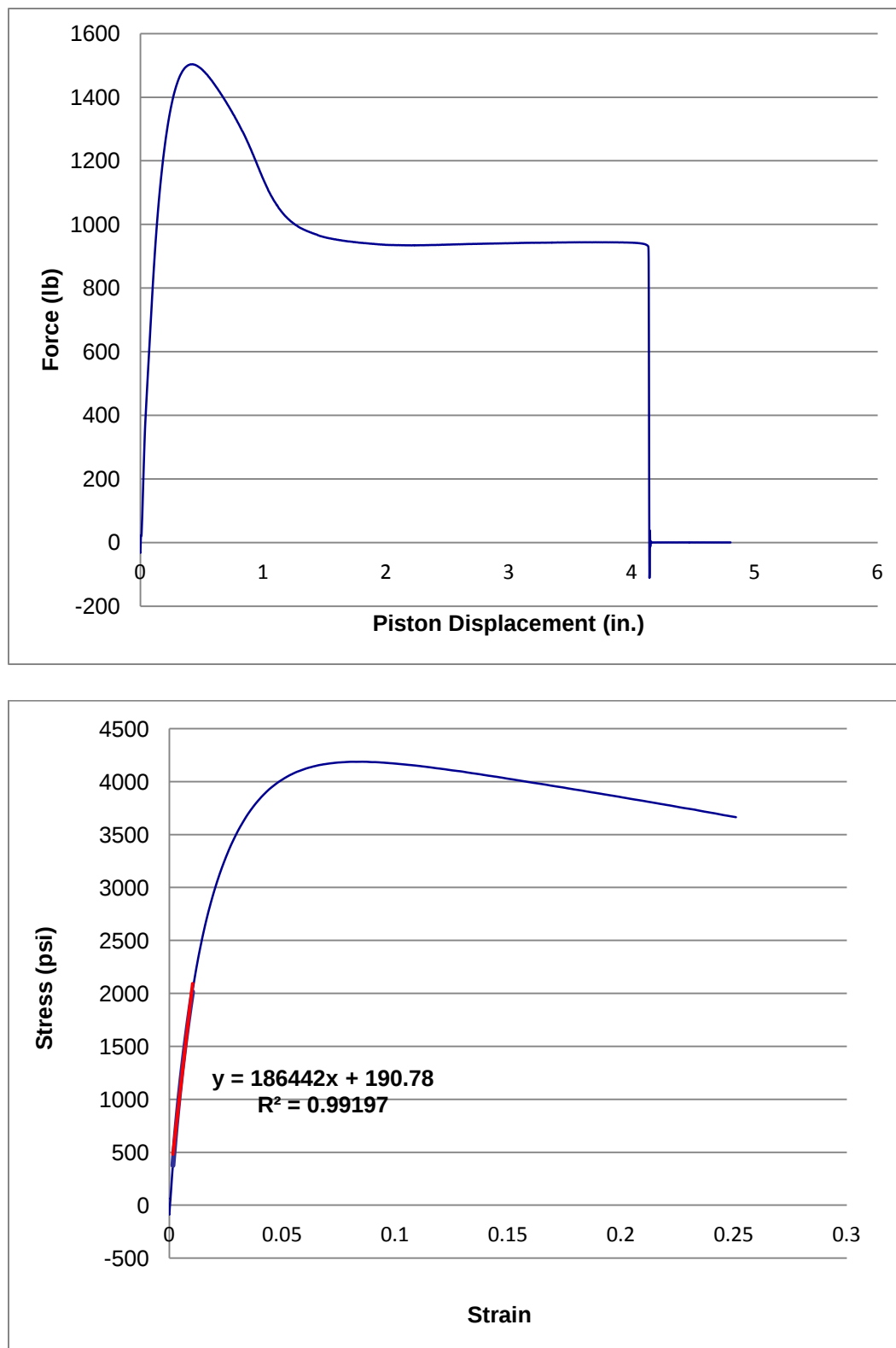
Figure 6. Typical force-displacement plot ( upper ) and stress-strain plot ( lower ) for Vendor B HMW-PE specimens (specimen B-21: 23 °C and 20 in./min). Tensile stress at yield was the maximum stress for all test specimens.
