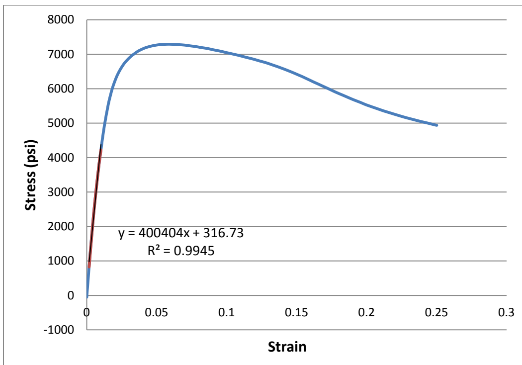
Figure E4. Stress-strain plot for Vendor B sample BFS-1. Piston controlled at -40^{\circ}\text{C} and 20 in./min crosshead speed illustrating Young's modulus calculation.
