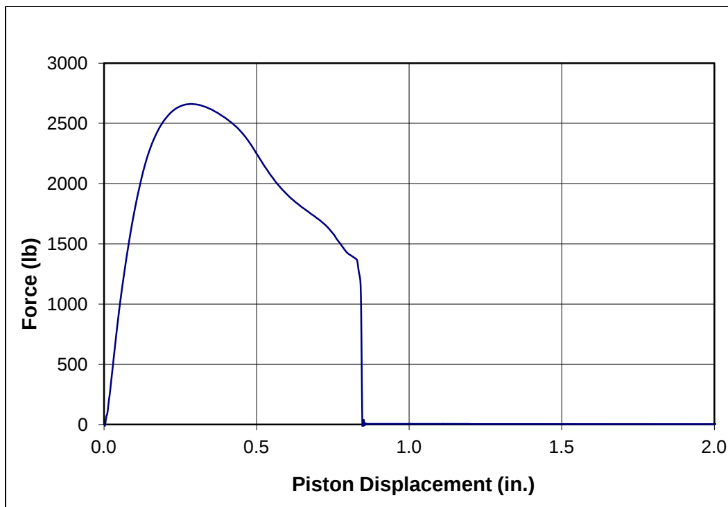
Figure E3. Force vs. piston displacement for Vendor B sample BFS-1. Piston-controlled load-displacement plot at -40^{\circ}\text{C} and 20 in./min crosshead speed.
