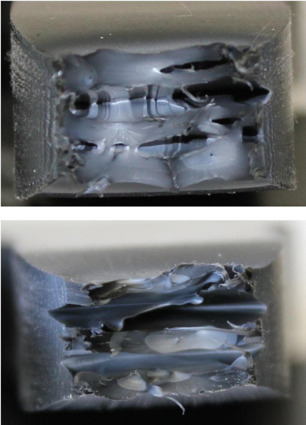
Figure 16. Splitting and crazing of Vendor A HMW-PE at failure surfaces of a new, unused specimen ( upper ) and a field specimen ( lower ) tested at -40^{\circ}\text{C} and 20 in./min.
