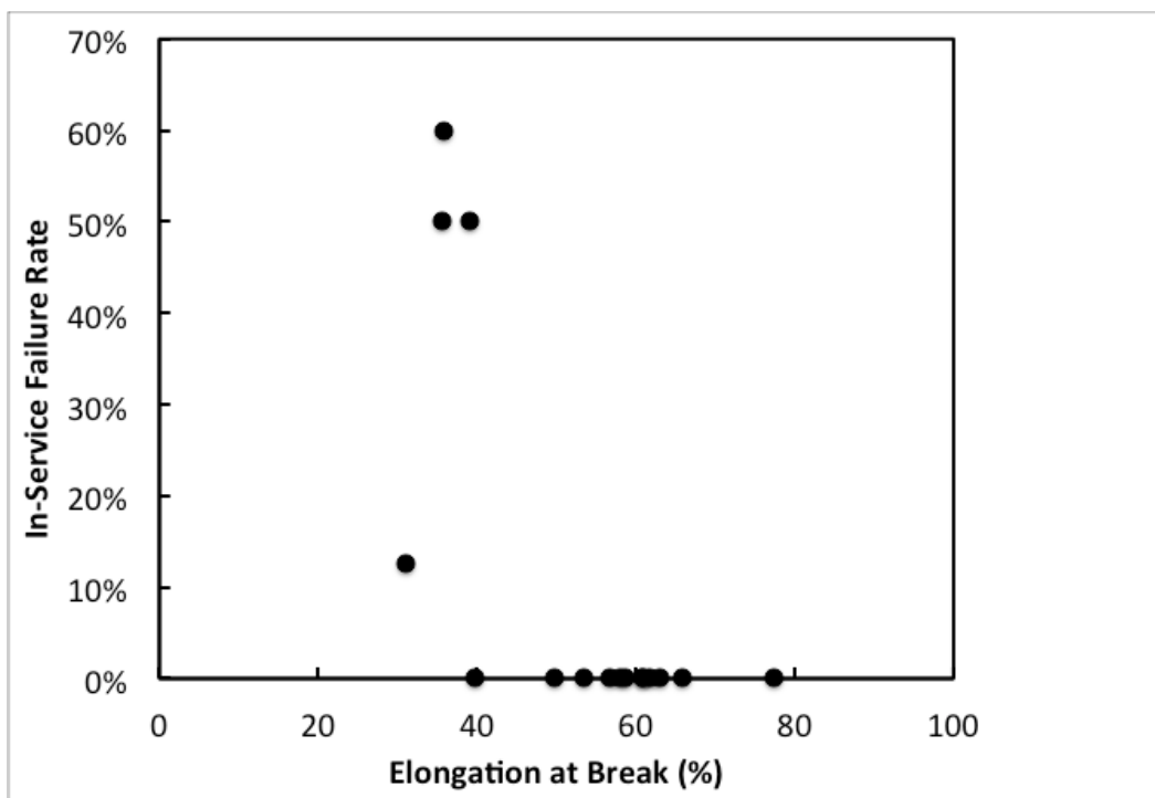
Figure 19. In-service sled failure rates versus elongation at break for specimens obtained prior to the field season. The results are for all production runs of HMW-PE tested and for SPoT and GrIT in-service failures.
