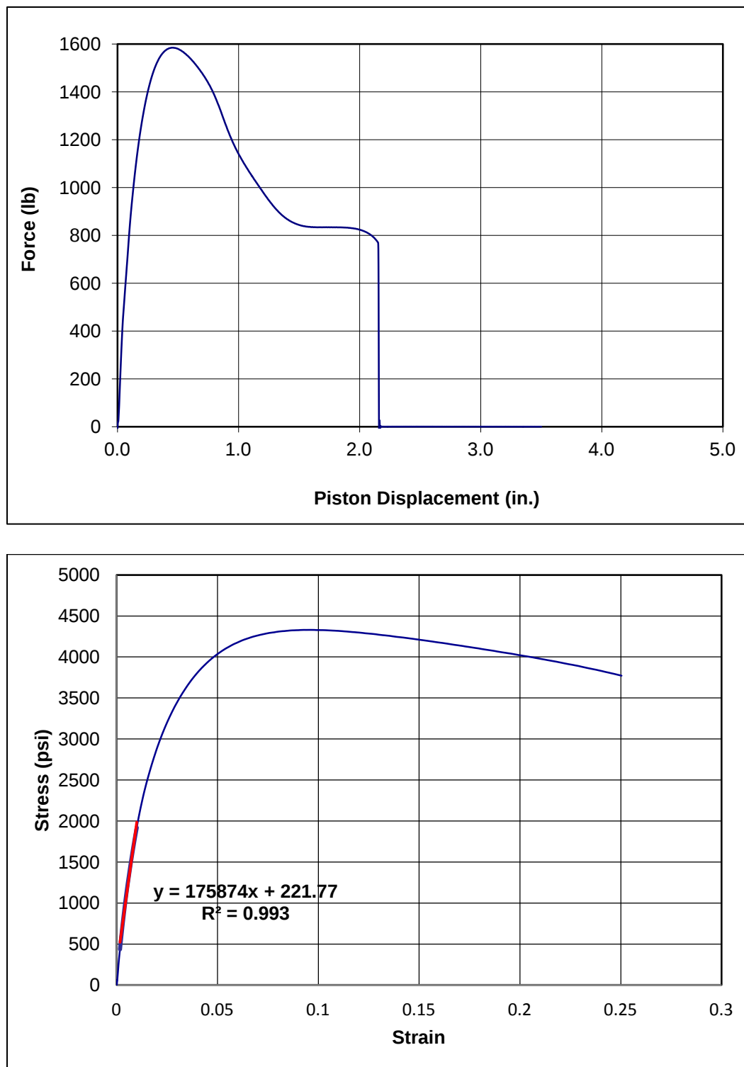
Figure 5. Typical force-displacement plot ( upper ) and stress-strain plot ( lower ) for Vendor A HMW-PE specimens (specimen A-22: 23 °C and 20 in./min). Tensile stress at yield was the maximum stress for all test specimens.
