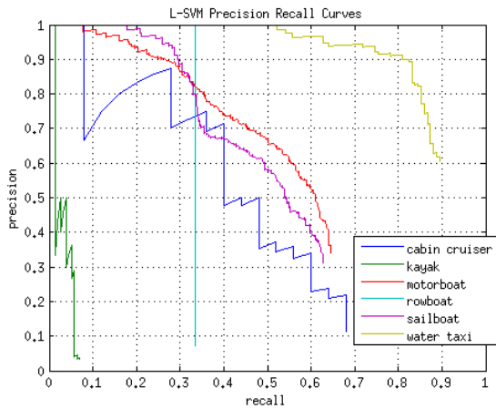
Figure 5. Precision-Recall performance graphs for L-SVM and E-SVM . Category water_taxi is the best performing maritime vessel category for all three object detection algorithms. Smaller class vessels such as kayak performed poorly.
