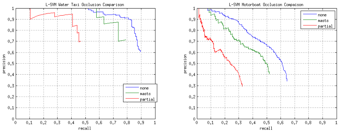
Figure 7. As expected, maritime vessels with the least occlusion are more easily detectable than vessels that suffer from obstruction.
