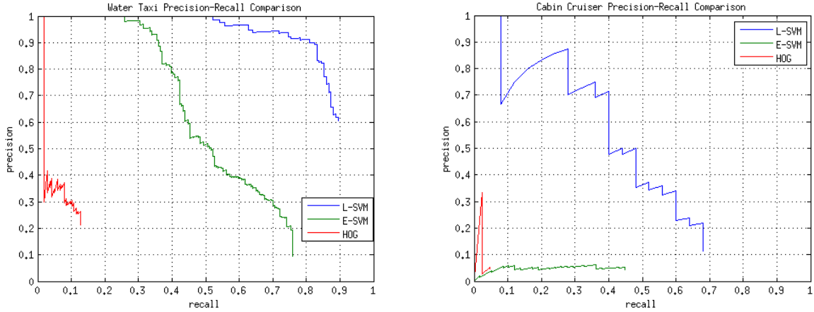
Figure 6. Performance comparison of the three object detection algorithms of two maritime vessel categories ( water_taxi and cabin_cruiser ). L-SVM is the best performing algorithm with the highest average precision rating on all six categories.
