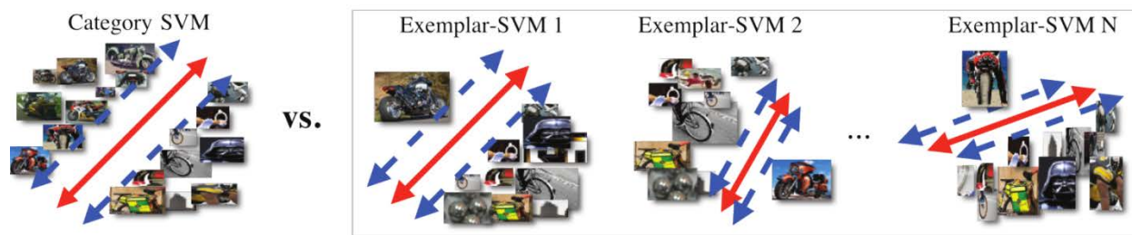
Figure 2. This shows the main difference between a general SVM and Exemplar-SVM . In a general SVM, multiple instances of the object are trained together as positives while in E-SVM , only a single instance of the object (usually of a certain pose) is trained. The three positives shown in Exemplar-SVM represent different view profiles of the motorcycle.
