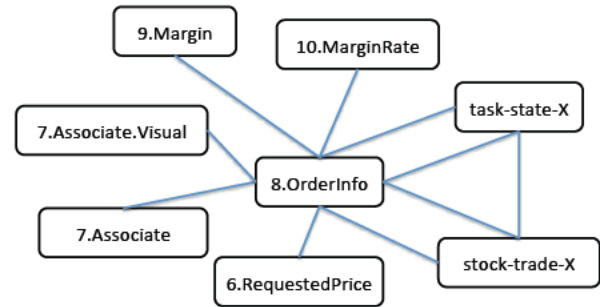
Figure 3: Illustrative associations for the eighth step of the stock trader experiment, Order Info. “Task-state-X” is a placeholder for various episodic codes associated with Order Info over time. “Stock-trade-X” is a placeholder for various goals associated with Order Info over time; episodic codes are associated with the goal in working memory that they co-occur with. Other associations are made, as well, but for clarity we omit those not relevant to our discussion.
