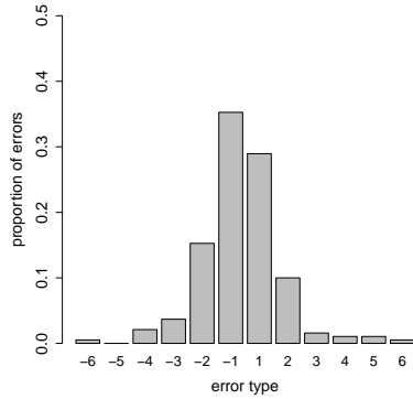
(b) Distribution of sequence errors after an interruption in a horizontal interface. Note the higher proportion of +/-2 errors, and wider distribution spread, that occur.
