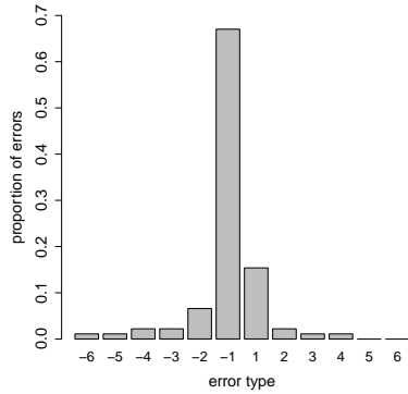
(a) Distribution of sequence error after an interruption in a columnar interface. Data is from Trafton et al., (2011).
