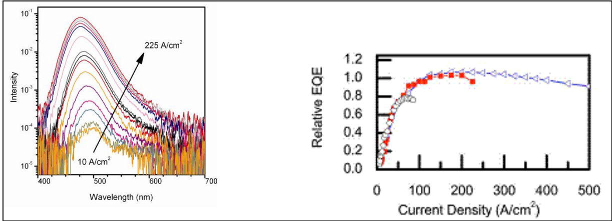
Figure 1. (a) The typical emission spectra at 10% duty cycle with respect to current density for an n\text{-In}_{0.22}\text{Ga}_{0.78}\text{N}/p\text{-Ga}_{0.5}\text{N} p -down, Ga-polar device, and (b) the relative external quantum efficiency (EQE) as a function of current density for cw (circles), 1% (triangles) and 10% (squares) duty cycle.
