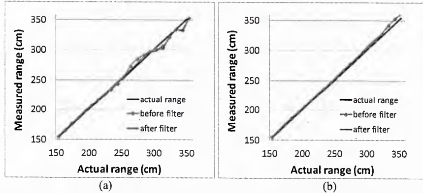
Figure 2. Measured target range vs. actual target range for modulation frequencies of 140MHz (a) and 160MHz (b) in turbid water ( c=2.5/\text{m} ). The 'before filter' data corresponds to the experimental data that was used as an input to the single delay line spatial filter, and the 'after filter' data is the resulting range after the spatial filter is applied.
