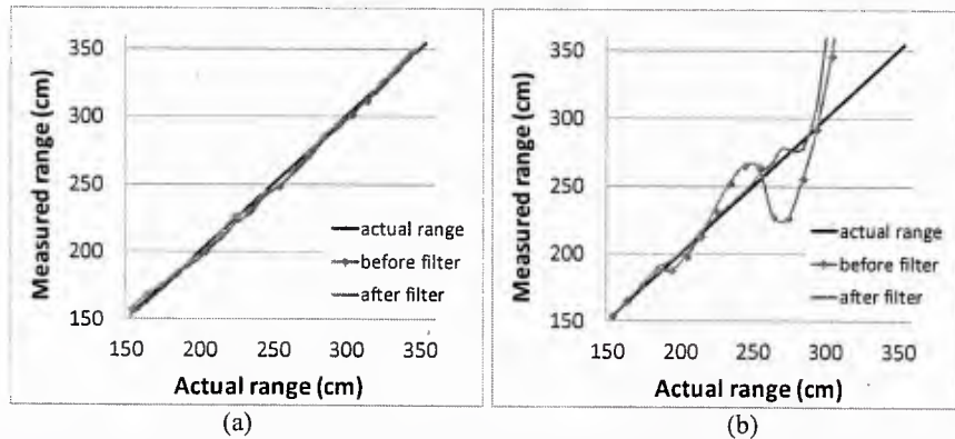
Figure 3. Measured target range vs. actual target range for the 'dual frequency' approach using modulation frequencies of 140MHz and 160MHz in clean water ( c=0.08/\text{m} ) (a) and turbid water ( c=2.5/\text{m} ) (b). The 'before filter' data corresponds to the experimental data that was used as an input to the single delay line spatial filter, and the 'after filter' data is the resulting range after the spatial filter is applied.
