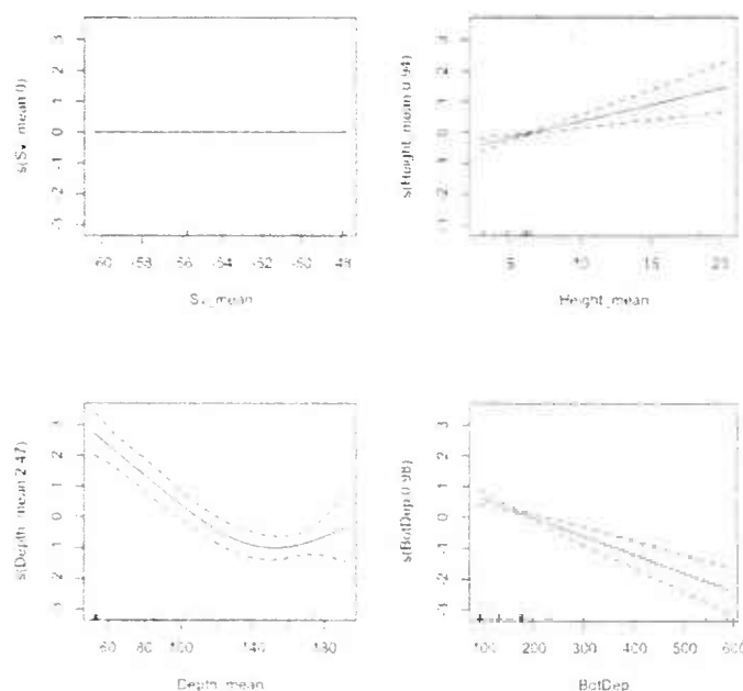
Figure 4. Dive axis 1 generalized additive mixed model output showing how dive behavior changes significantly as prey patches change.
