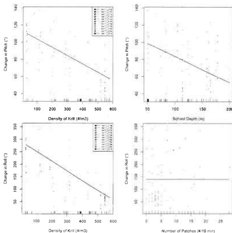
Figure 3. Relationships between changes in pitch (top) and roll (bottom) in blue whale feeding behavior as a function of krill density (#/m3), krill patch depth, and the number of krill patches measured.
