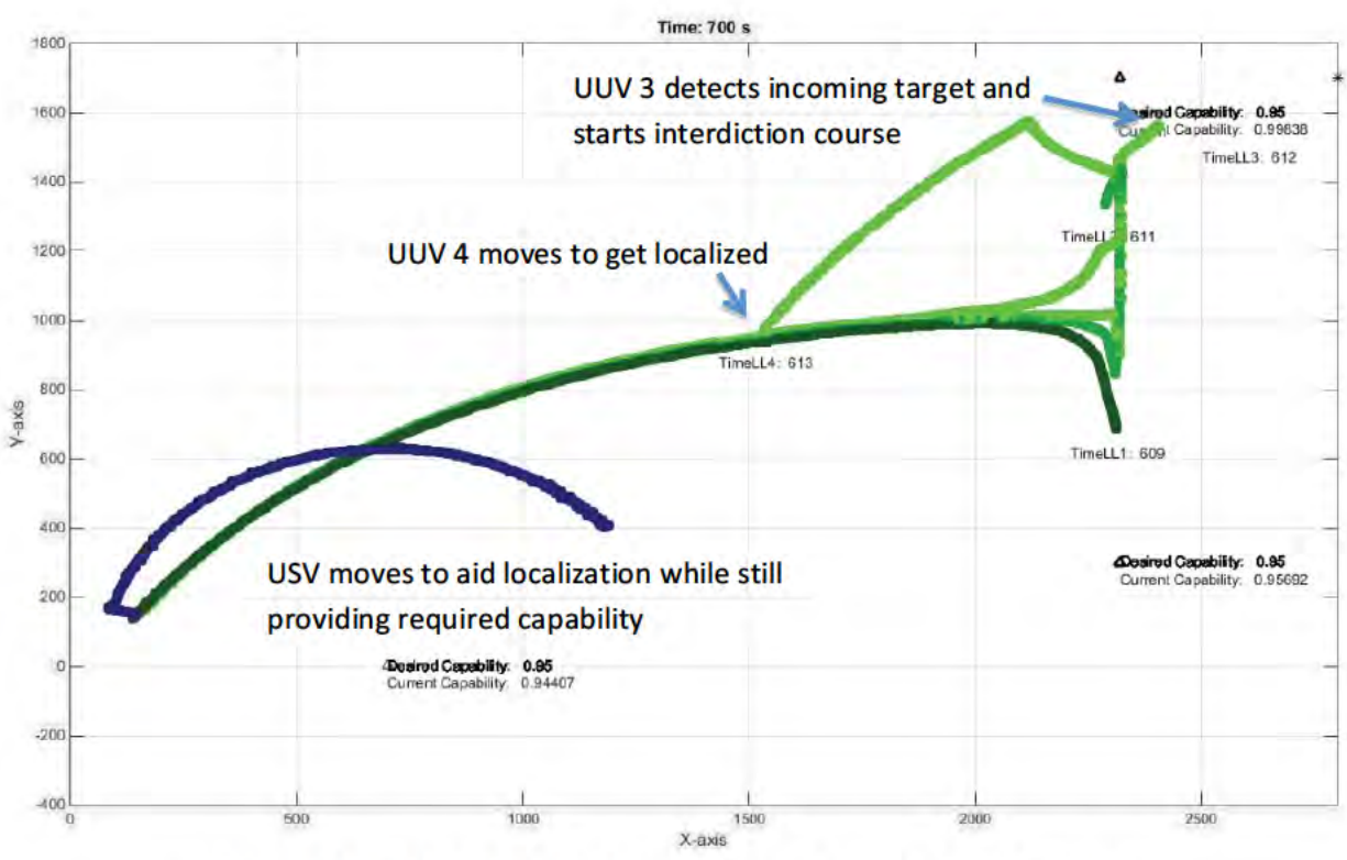
Figure 10.5: 4 UUV 1 USV Simulation with Interdiction (t = 700s)
