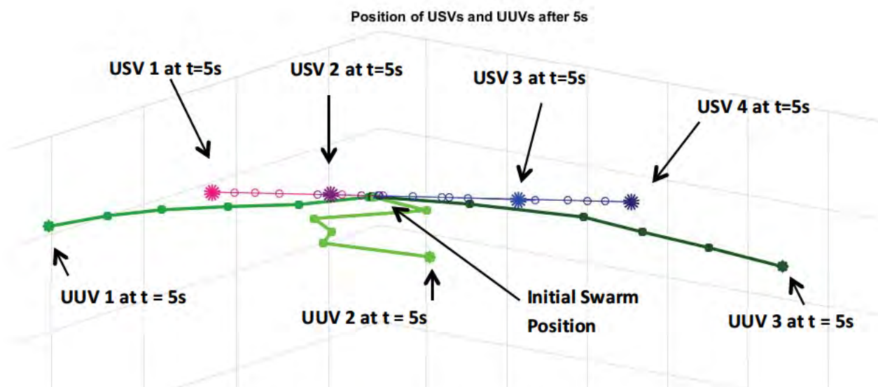
Figure 8.4: Position of USVs and UUVs after T = 5s
